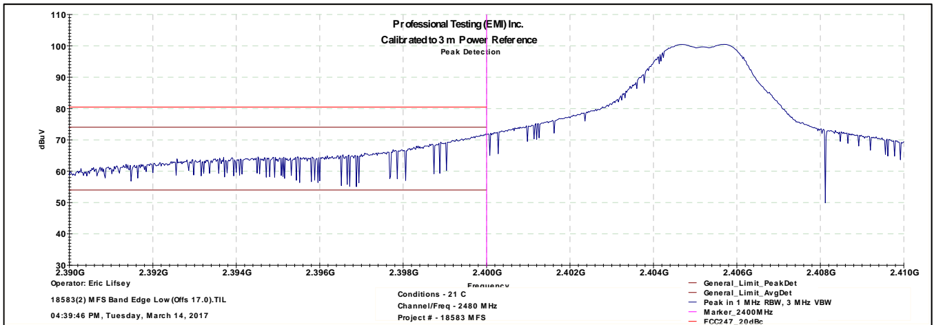
The 15.247 (-20 dBc) and general emission limits are shown.
