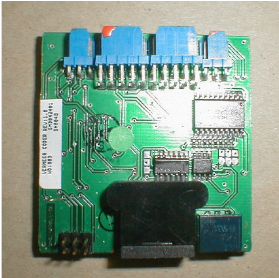
Vermeer Coder PCB Top View
