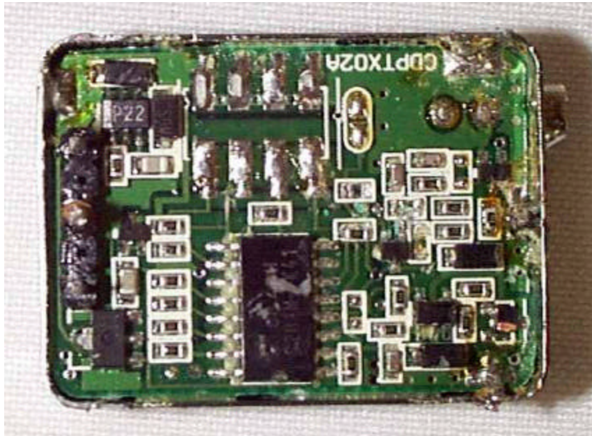
Transmit Module Removed From Mounting PCB, Bottom View
