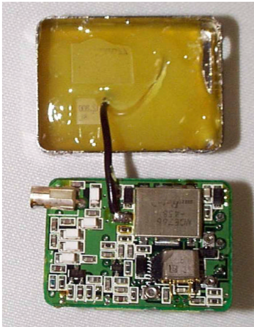
Transmit Module Removed From Mounting PCB, Cover Removed- Top View
