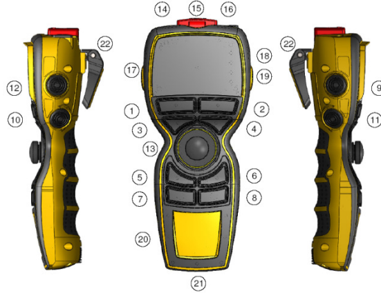
Figure 2. ERGO-S Transmitter (Right, Front, Left)
