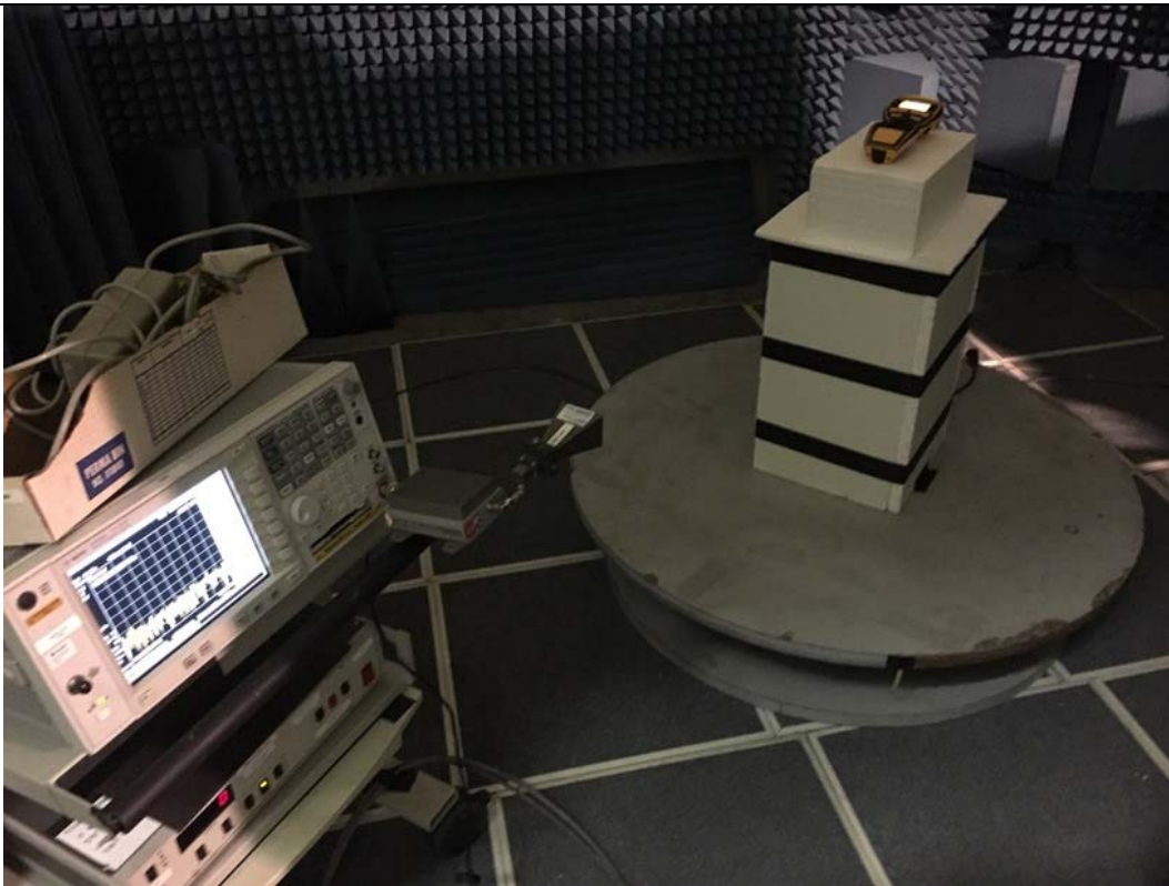
Radiated Emissions to 25 GHz;
