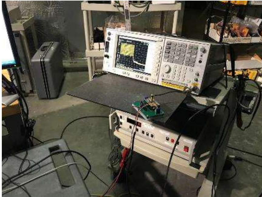
Conducted antenna port measurements; OBW, Power, Band Edge, Spurious, Timings
