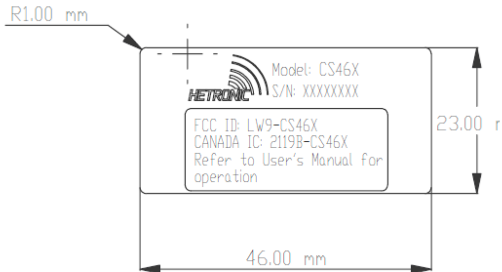
Figure 2, Module Label
