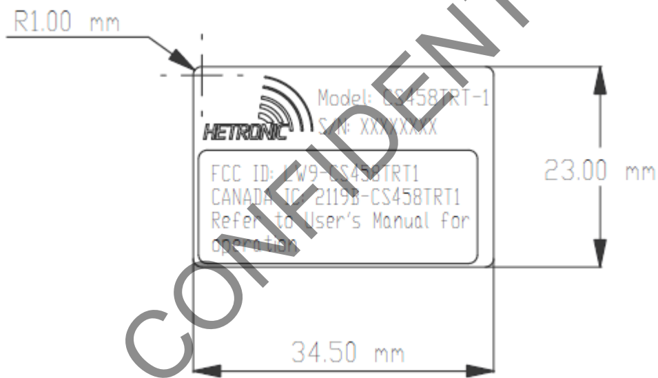
Figure 2, Module Label
