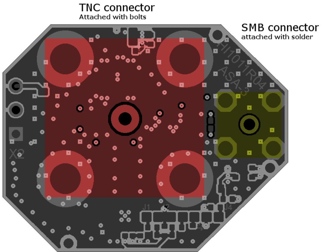
Figure 2, External RF connector placement, bottom side of PCB shown
