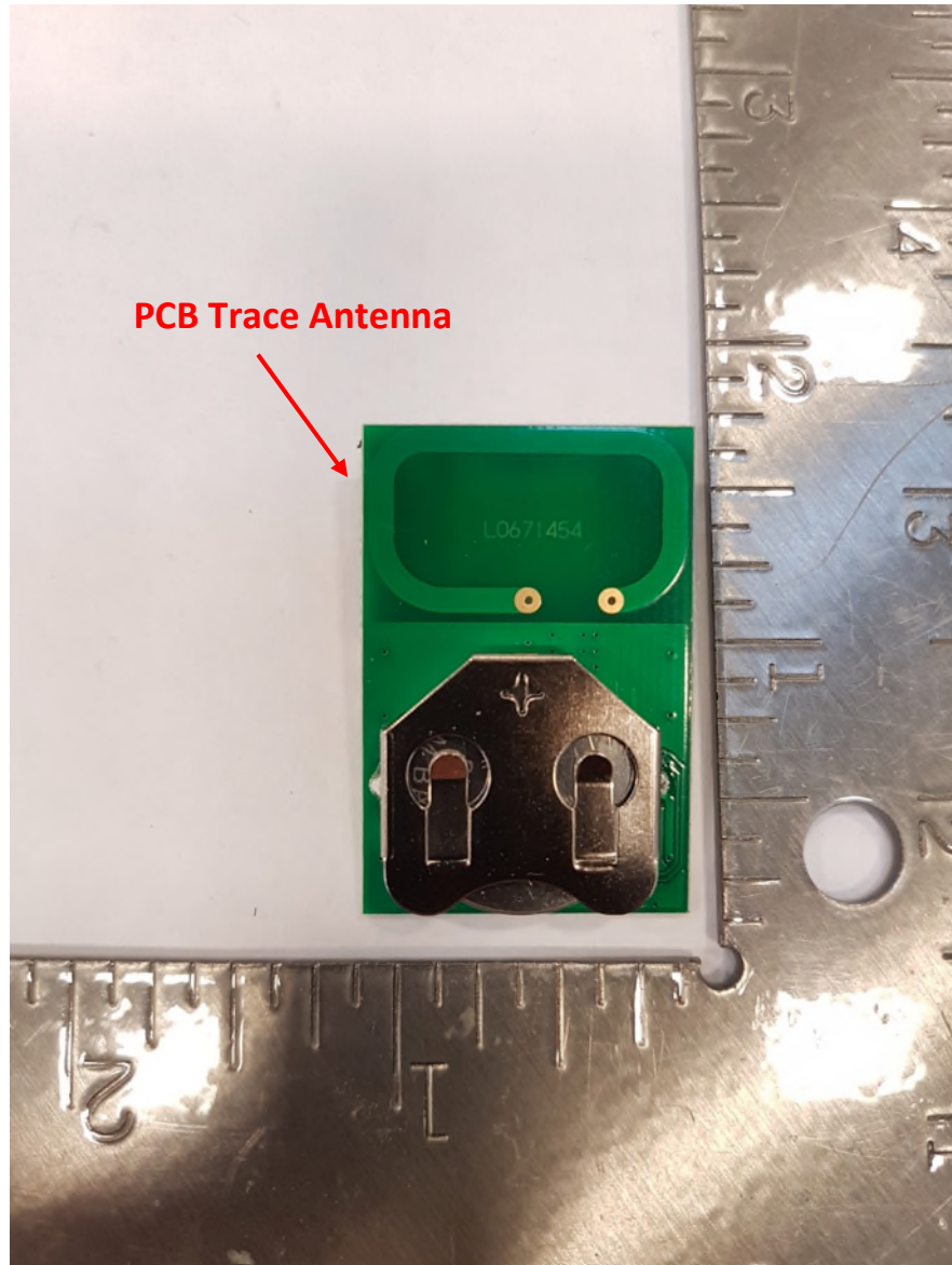
Figure 2 – EUT Internal Photo Back
