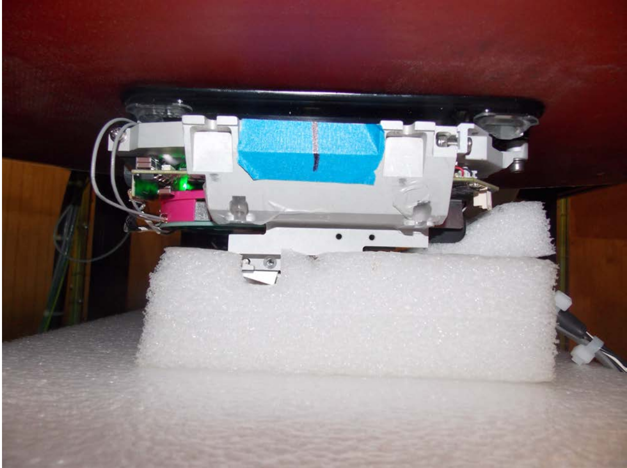
Test Position WiFi Test Position 0 mm Gap
