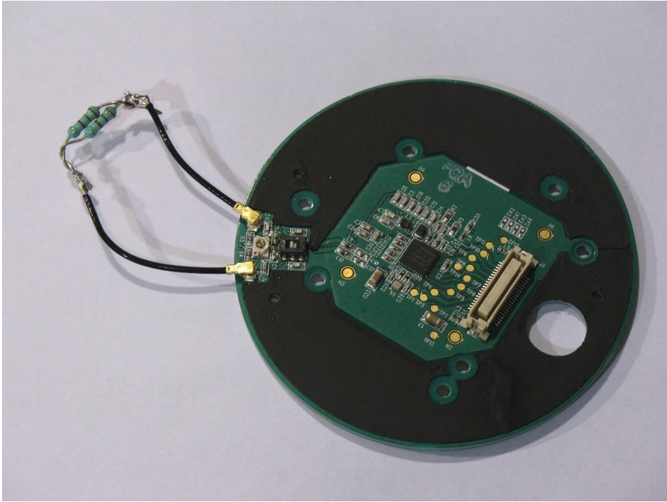
Dummy load conducted emissions configuration
