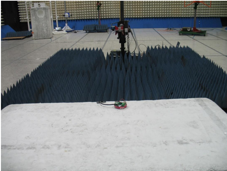
Radiated emissions 1-18GHz setup photo 2
