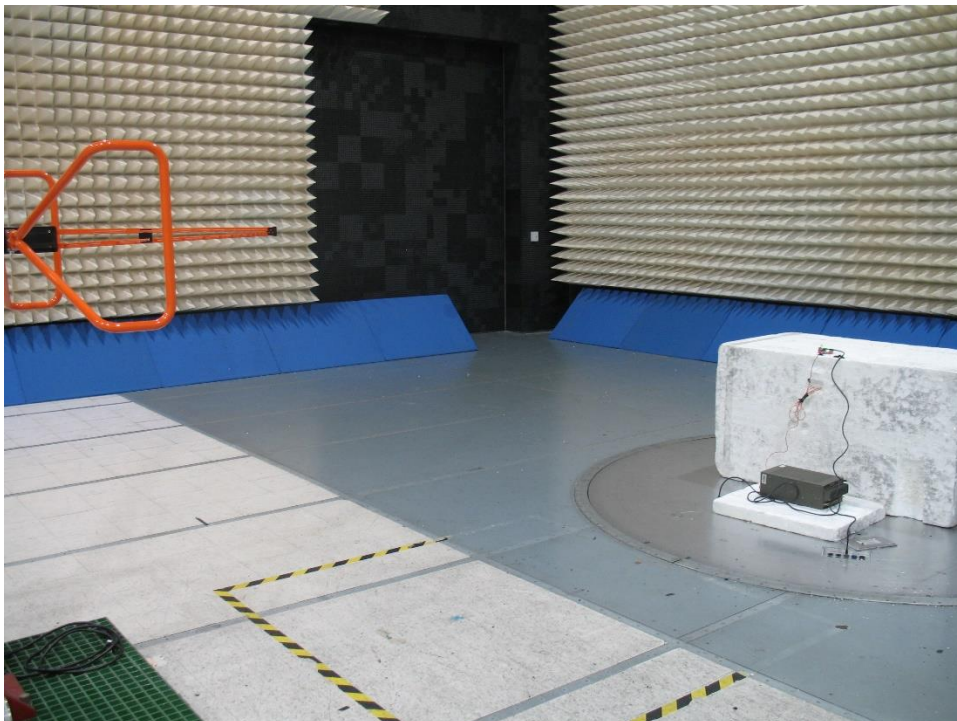
30MHz- 1GHz Test setup photo 2
