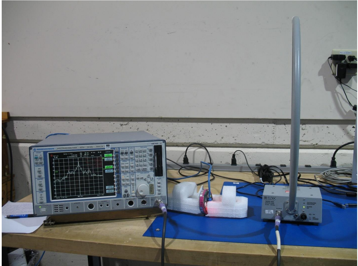
Occupied Bandwidth Setup Photo
