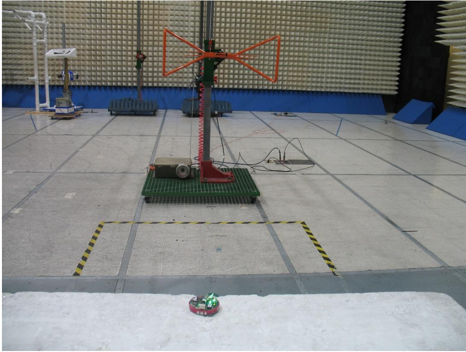
30MHz- 1GHz Test setup photo 1
