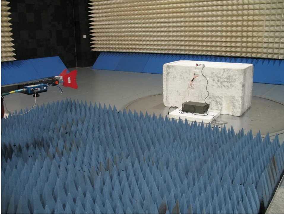
Radiated emissions 1-18GHz setup photo 1
