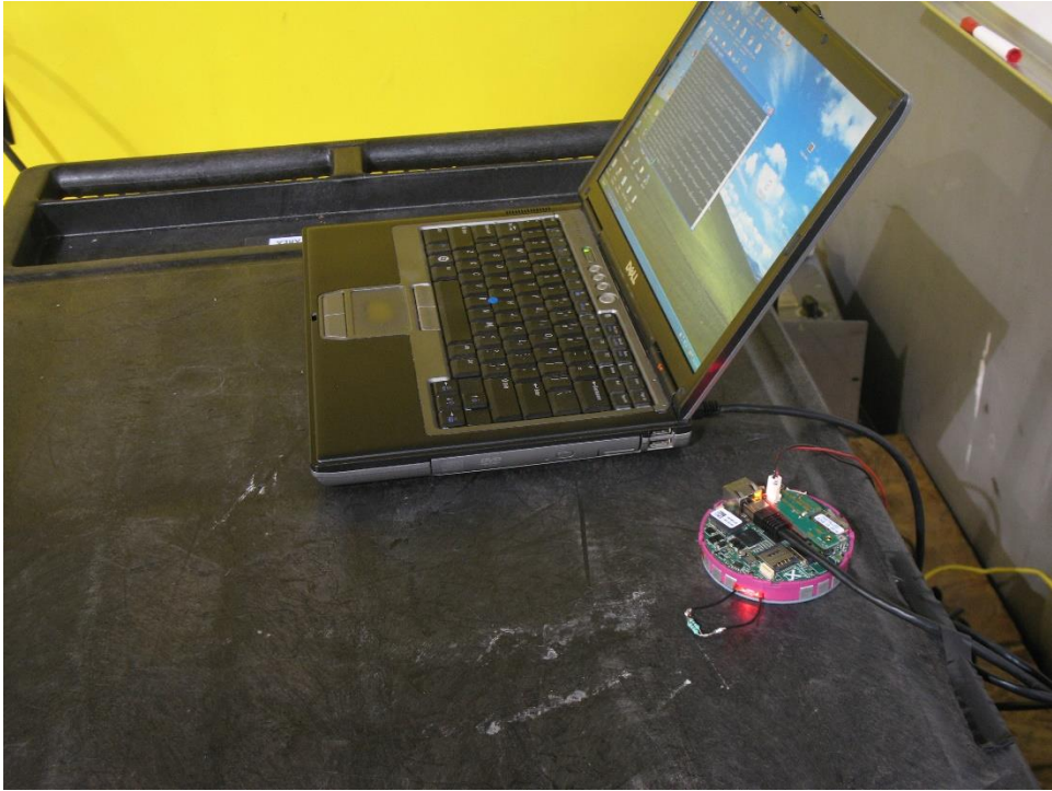
Dummy load conducted emissions test setup
