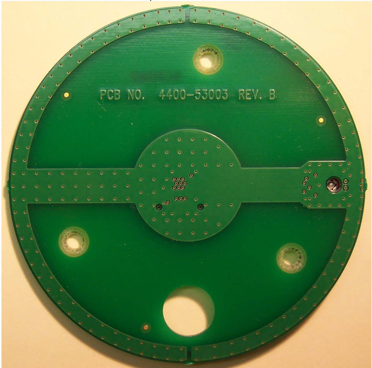
top of the antenna board
