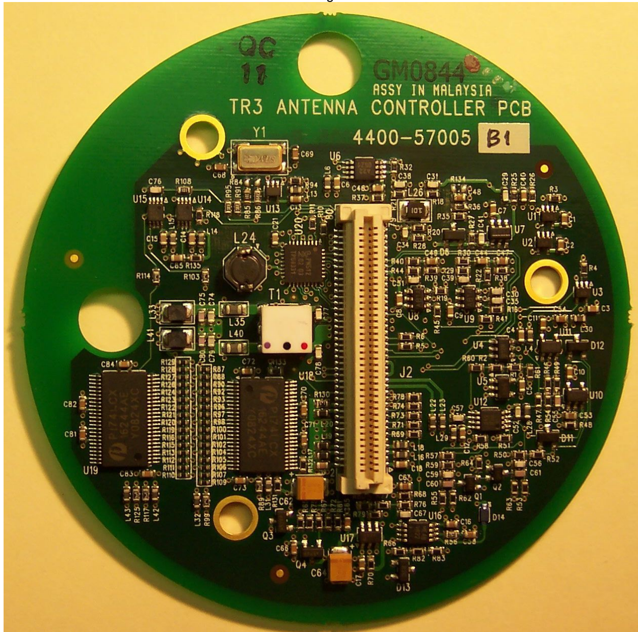
bottom of the analog controller board
