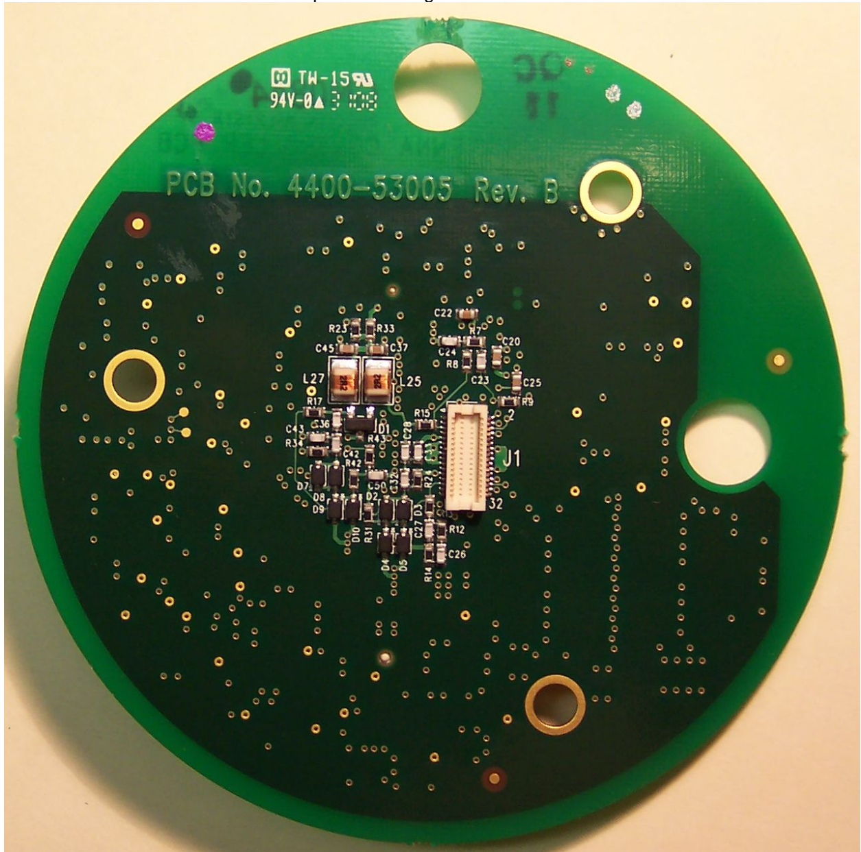
top of the analog controller board
