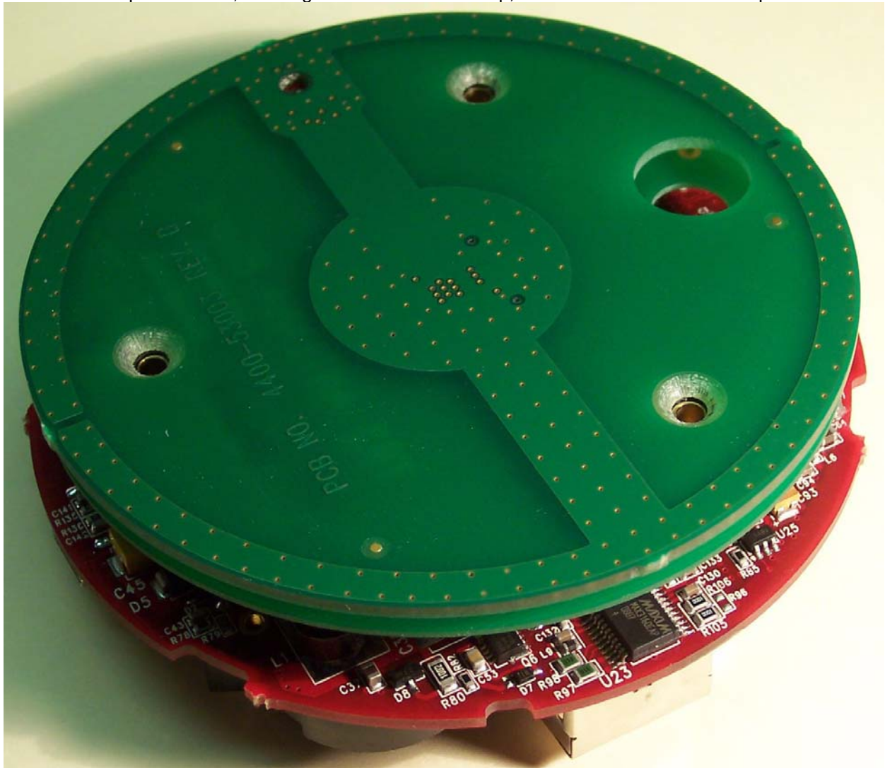
top of the TR3, showing the 3 boards staked up, with the antenna board on top.
