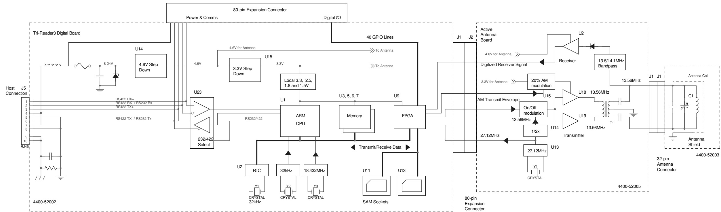
Tri-Reader3 Block Diagram
