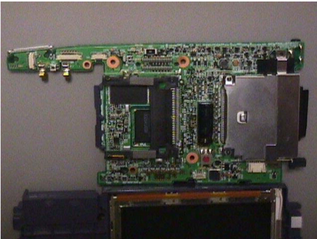
IT -70 M otherboard Side 2
