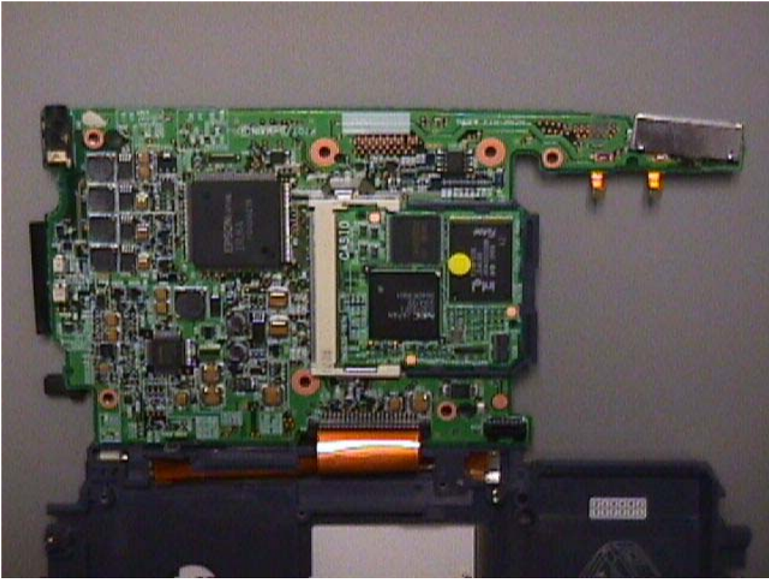
IT-70 Motherboard Side 1
