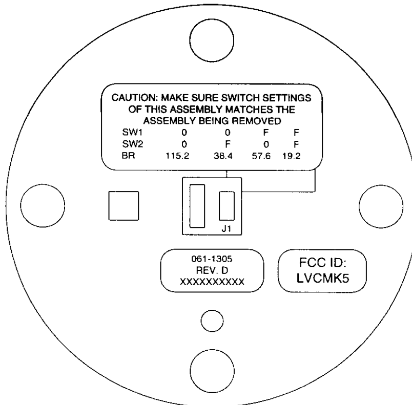
Target Labeling
