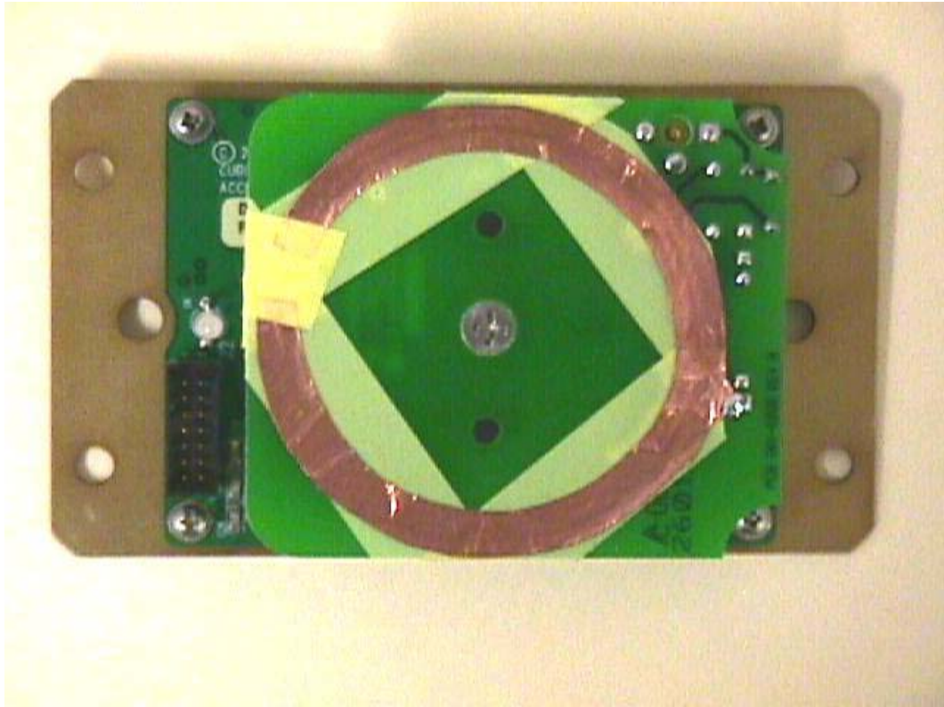
PCB ASSEMBLY 3
