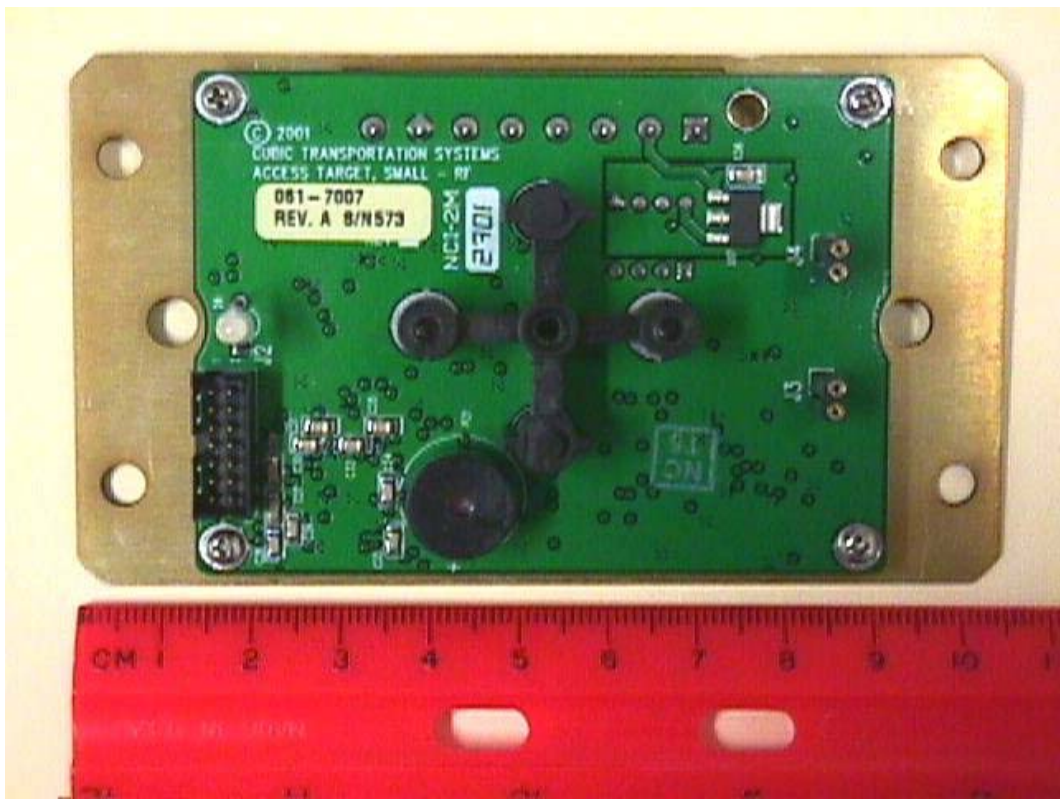
RF PCB SOLDER SIDE
