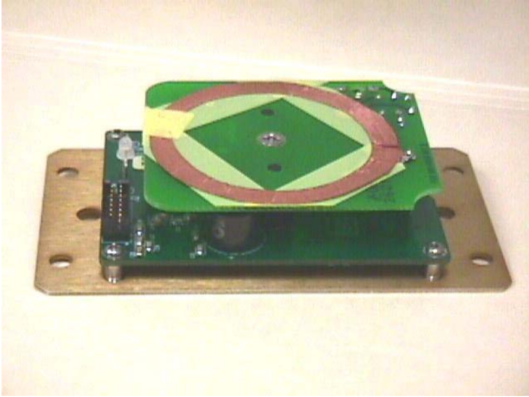
PCB ASSEMBLY 1
