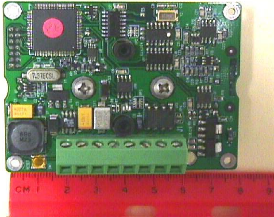
RF COMPONENT SIDE
