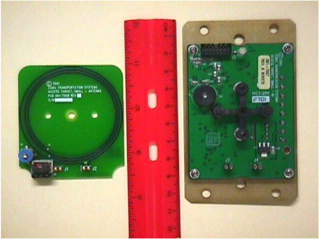
RF AND ANTENNA PCBs
