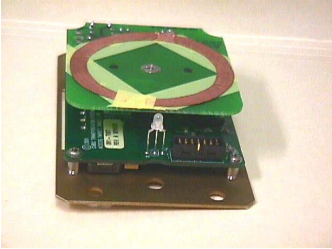
PCB ASSEMBLY 2
