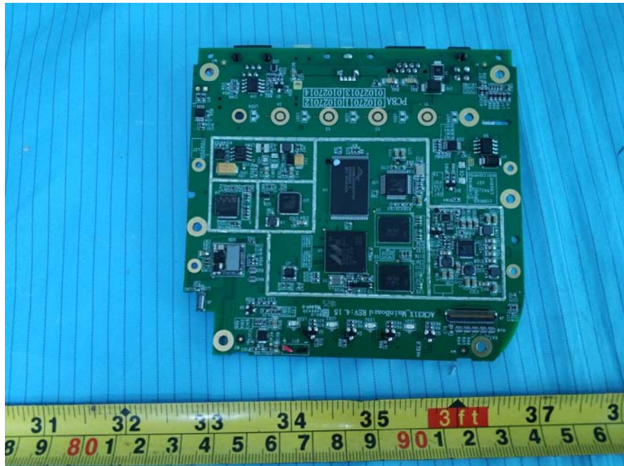
EUT – Main Board 3 Bottom View 3
