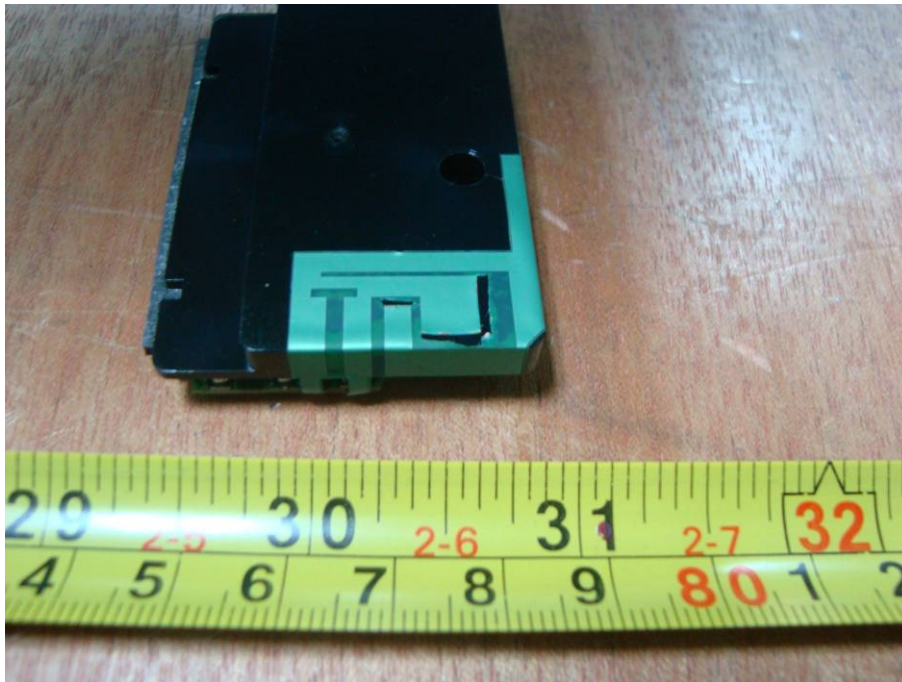
EUT – GSM/GPRS/EDGE/WCDMA Module Antenna Top View
