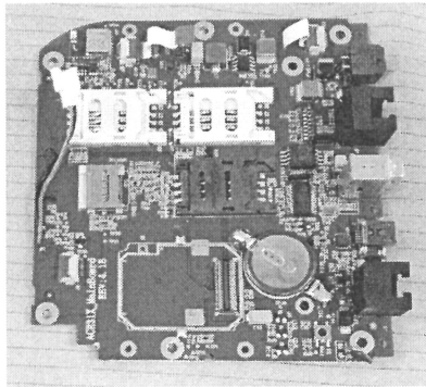
New board
