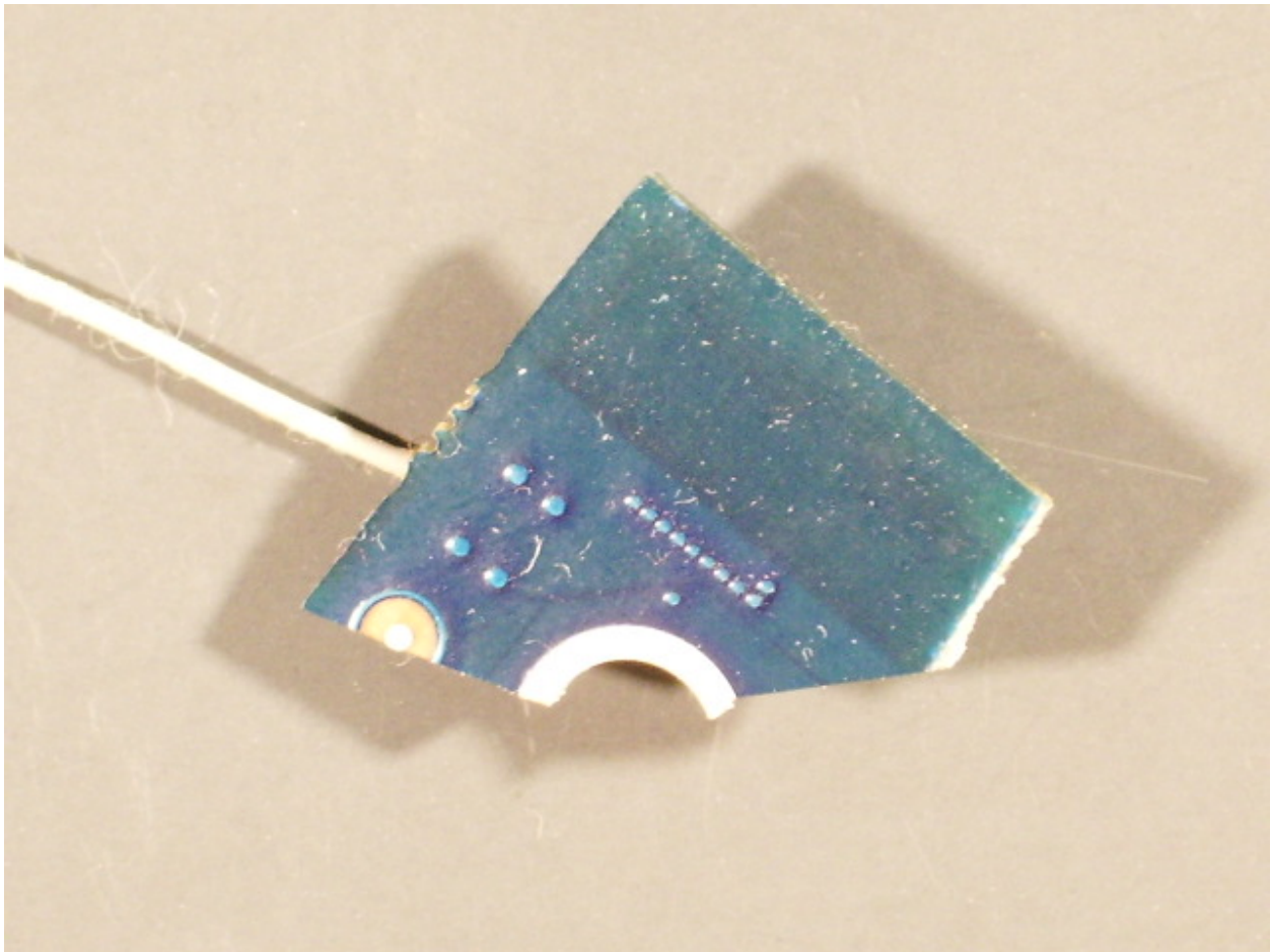
External Antenna - Bottom View
