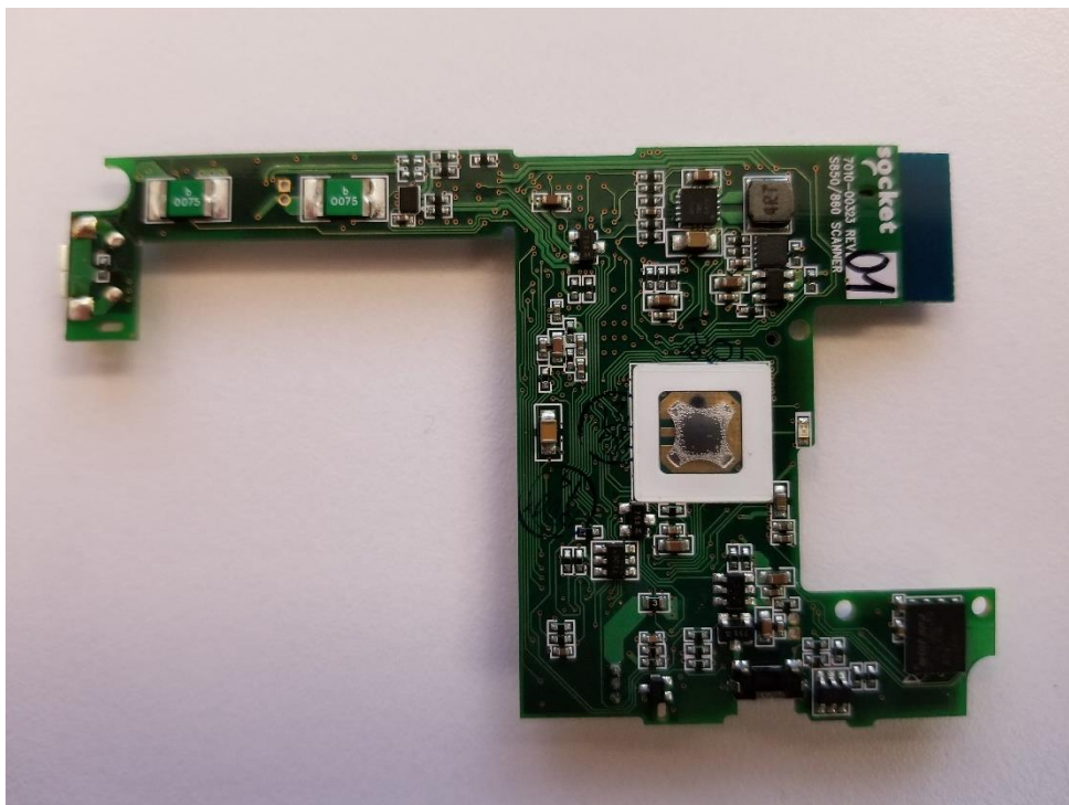
Model: S860 – Circuit Board – Bottom View
