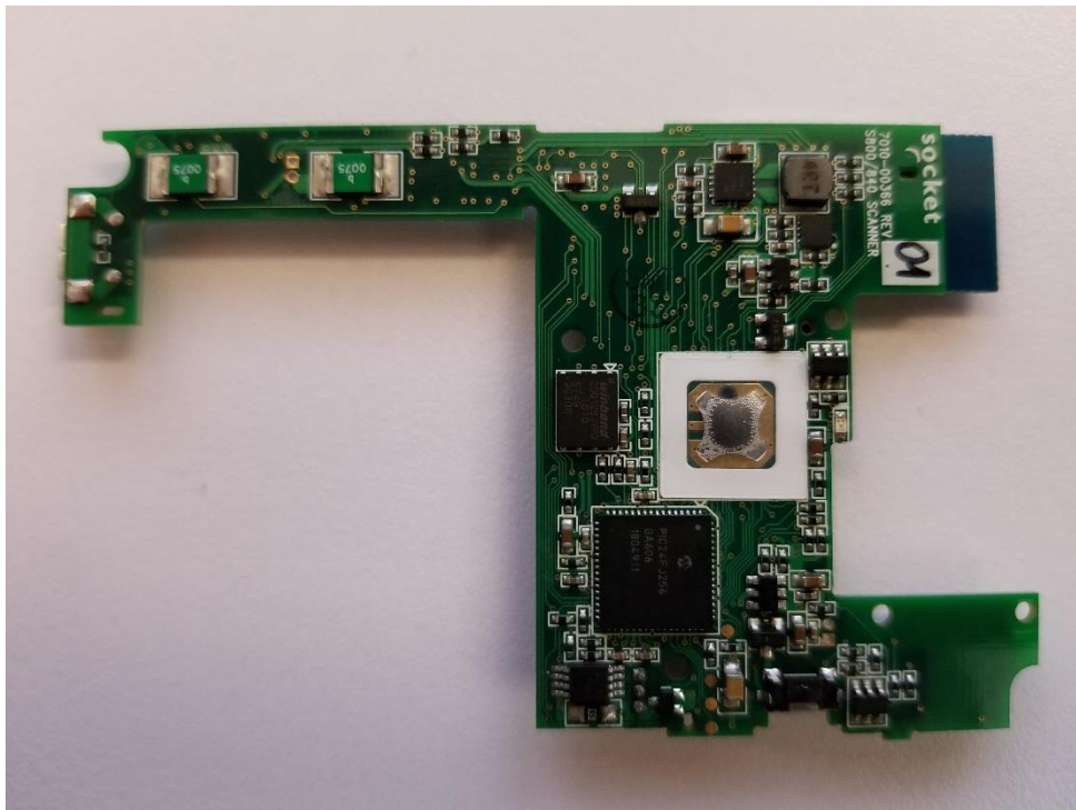
Model: S840 – Circuit Board – Bottom View
