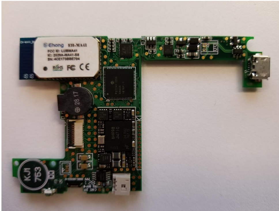
Model: S860 – Circuit Board – Top View
