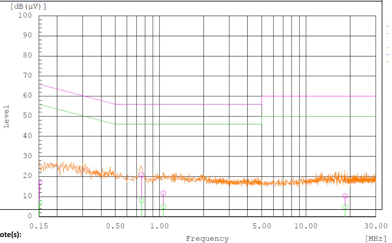
AC Line Conducted Emission (N) : RF output terminated with dummy load
