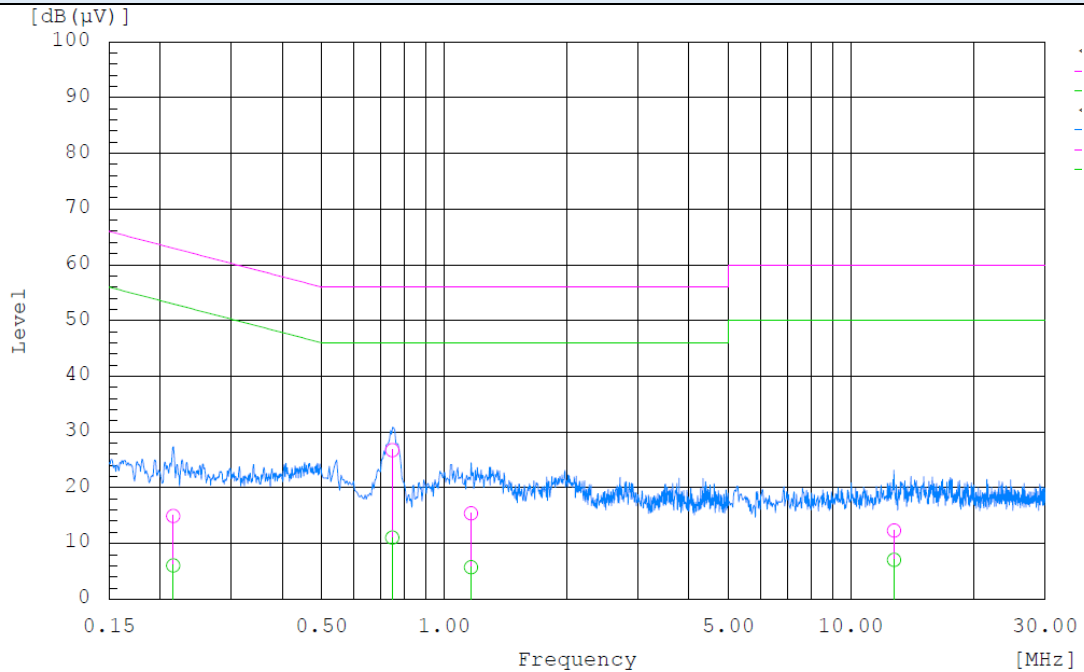
AC Line Conducted Emission (L1) : RF output terminated with dummy load
