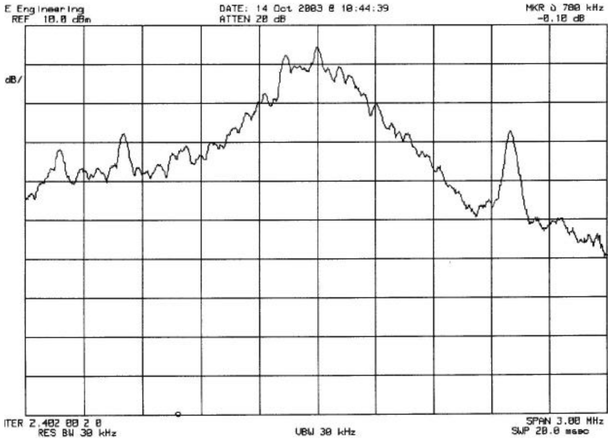
Plot 12: 20 dB BW 2402 MHz
