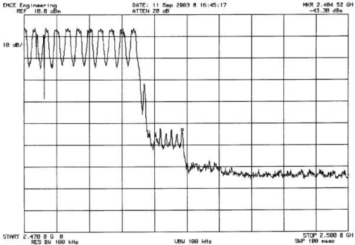
Plot 16: Band-edge compliance, (Upper Band-edge)
