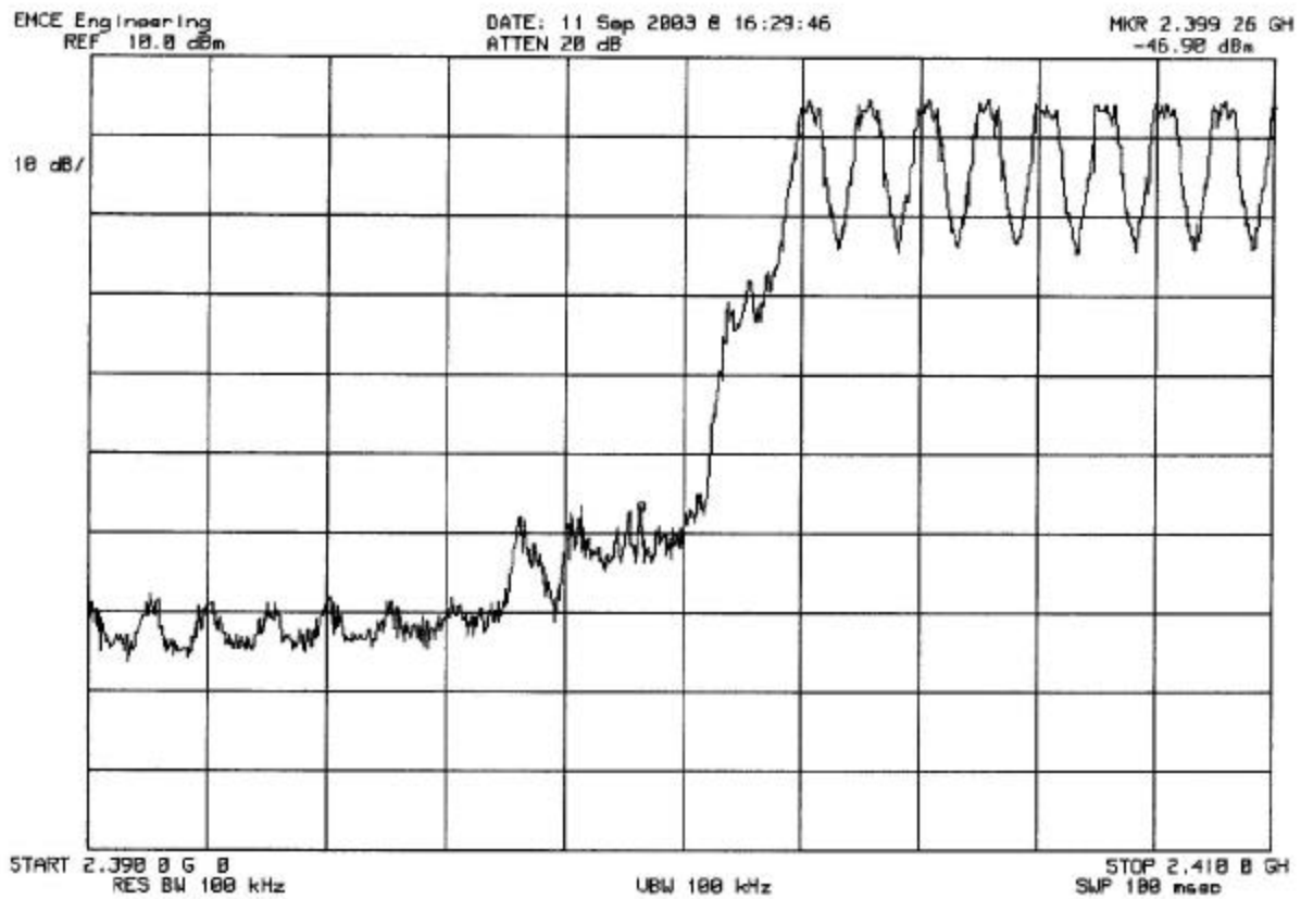
Plot 15: Band-edge Compliance, (Lower Band-edge)
