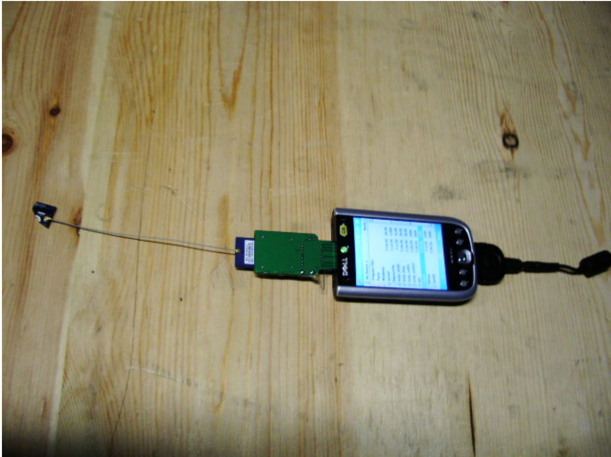
Modular Radiated Emissions Setup in SD Card Extender
