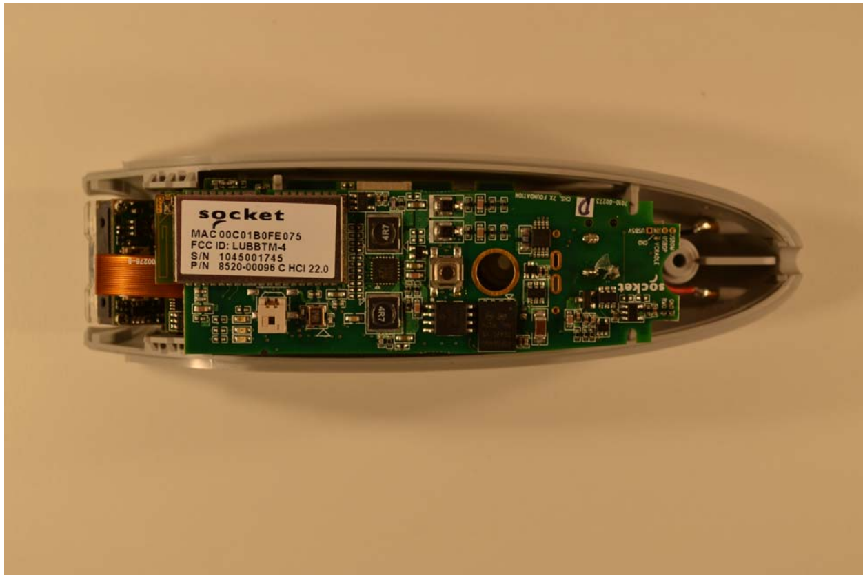
Main PCB – Top View
