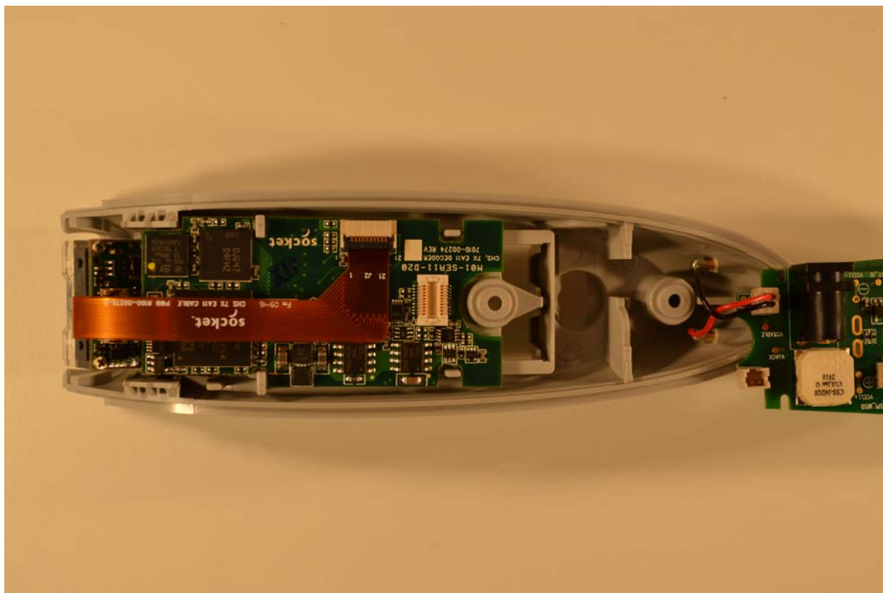
Radio PCB – Top View
