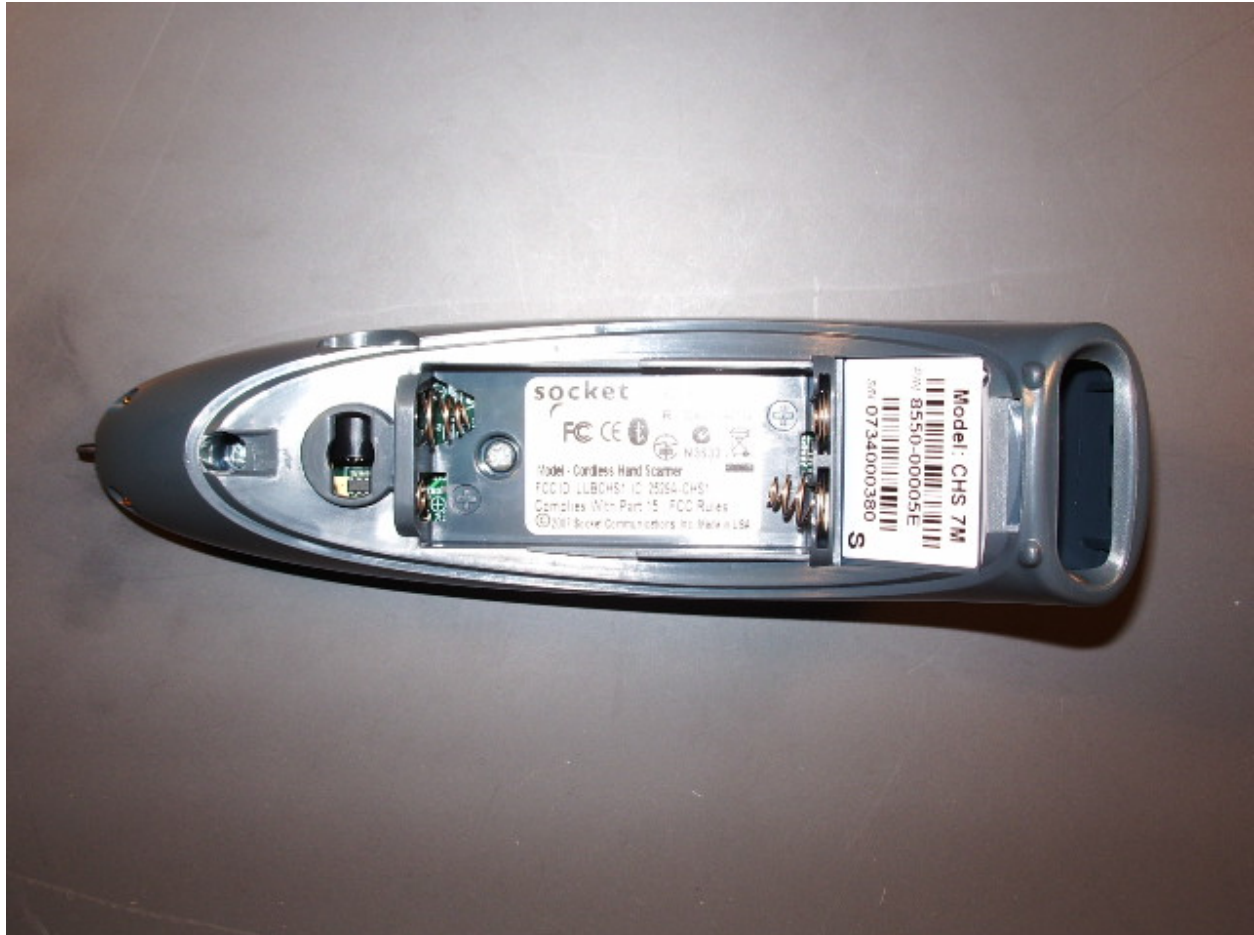
Enclosure Battery Cover Removed– Internal View
