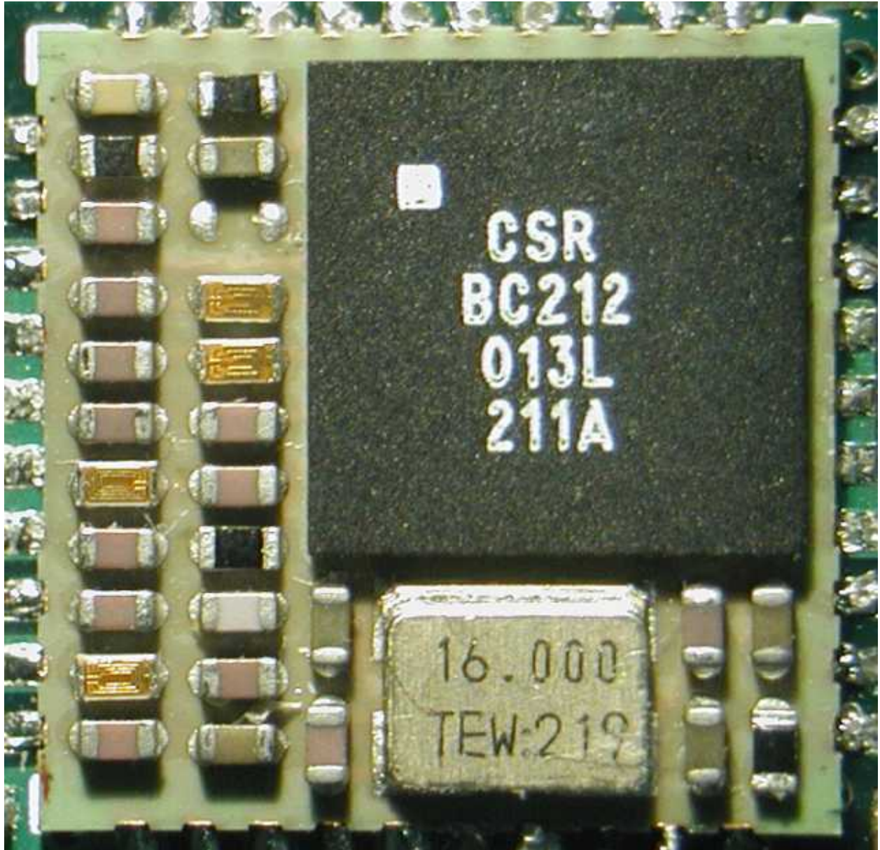
Radio Module – Internal View
