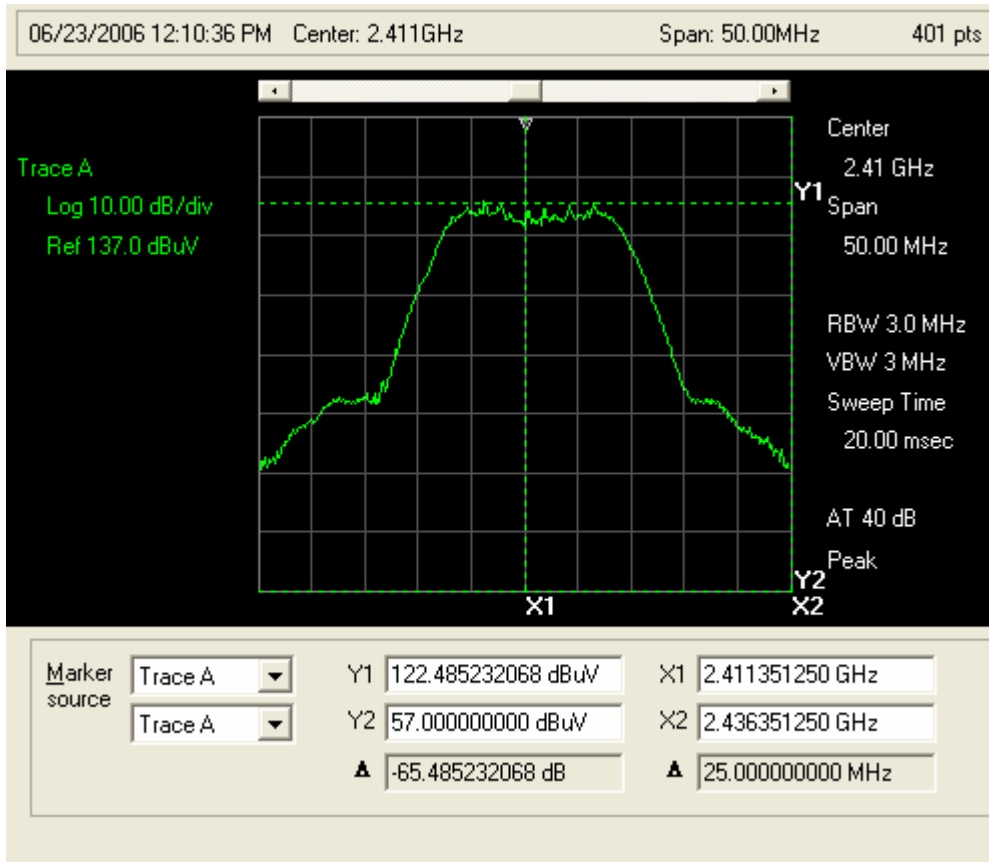
Plot 1: Peak output power 2412 MHz / 6 Mbit Modulation
