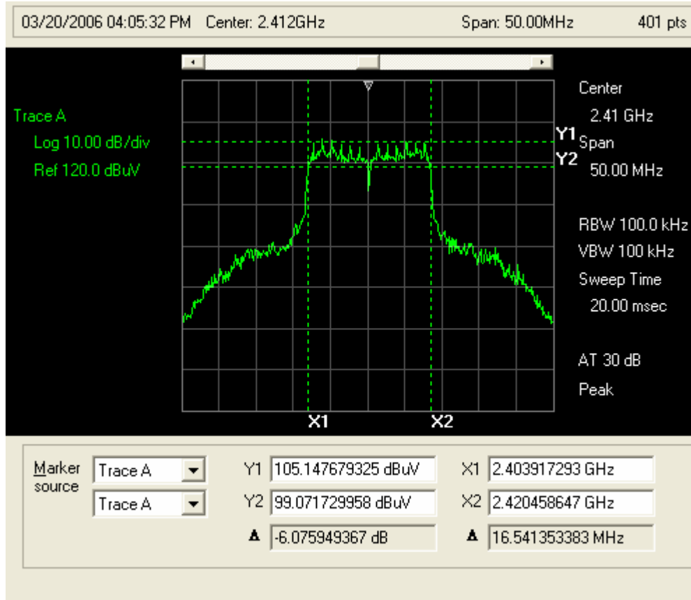
Plot 12: 6 dB BW 2412 MHz / 6 Mbit Modulation
