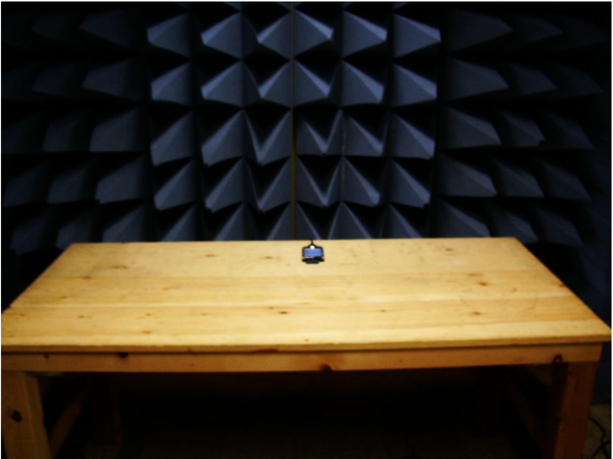
Radiated Spurious Emissions Setup
