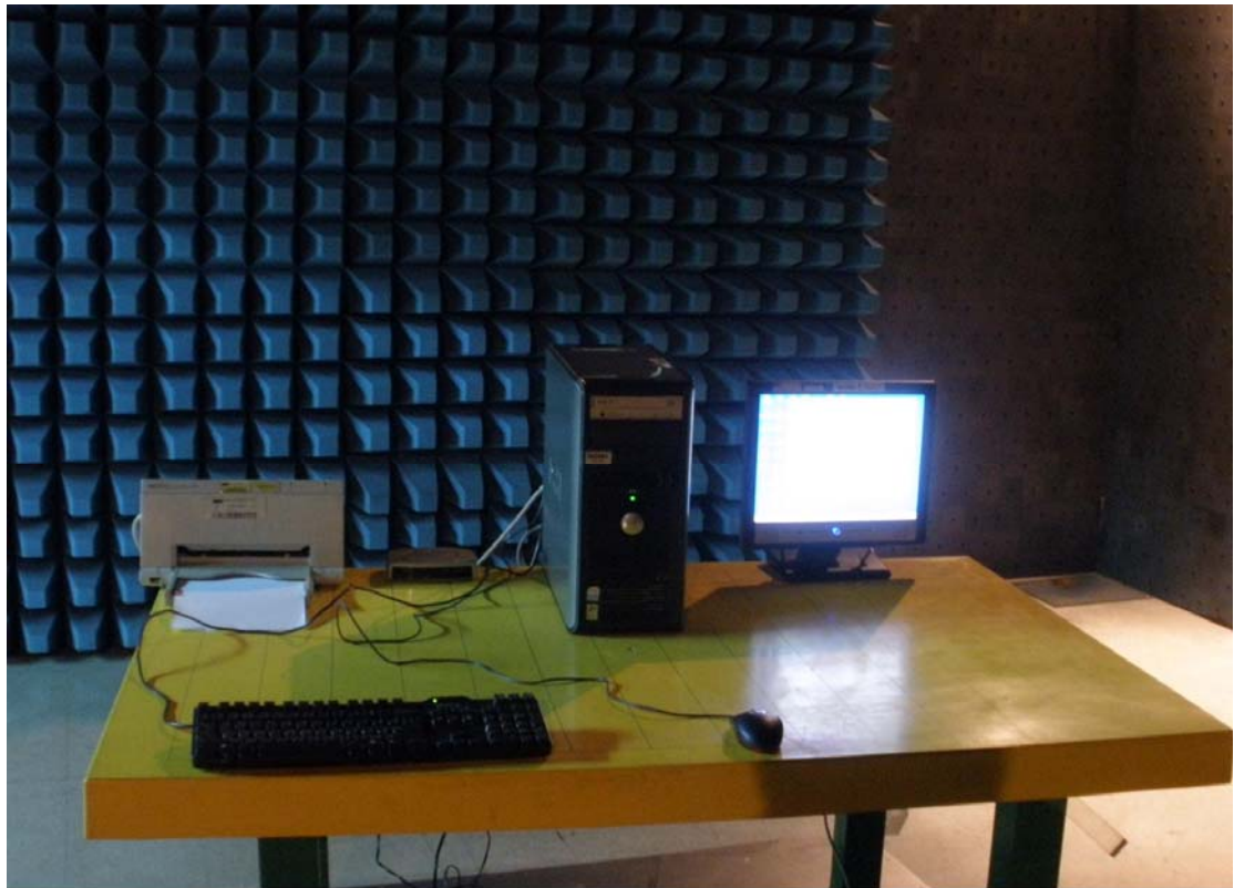
Photo 2: Radiated Emission Test set-up photo
