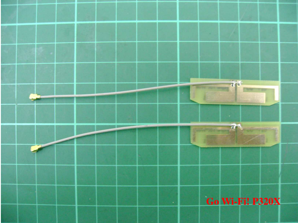
PCB antenna
