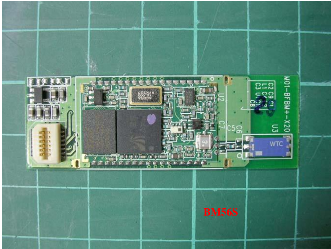
Photo 6: Internal photo of EUT (Bluetooth)
