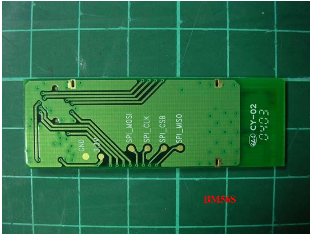
Photo 7: Internal photo of EUT (Bluetooth)
