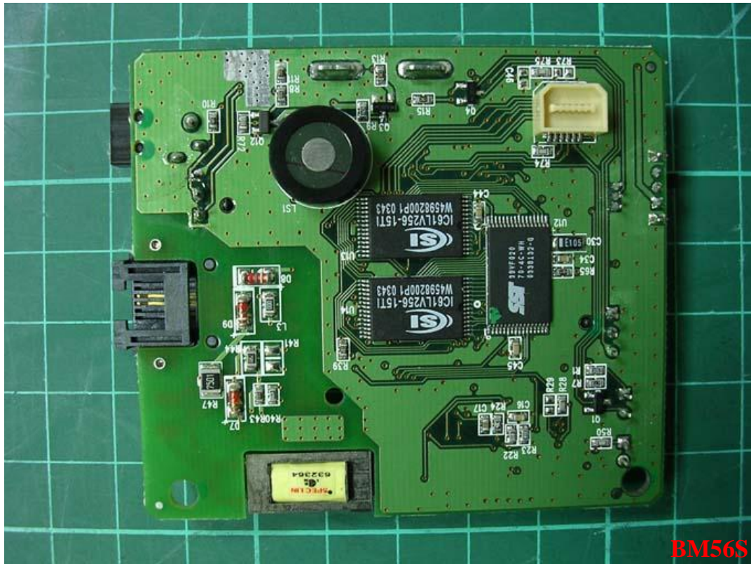
Photo 3: Internal photo of EUT (with transformer 1)
