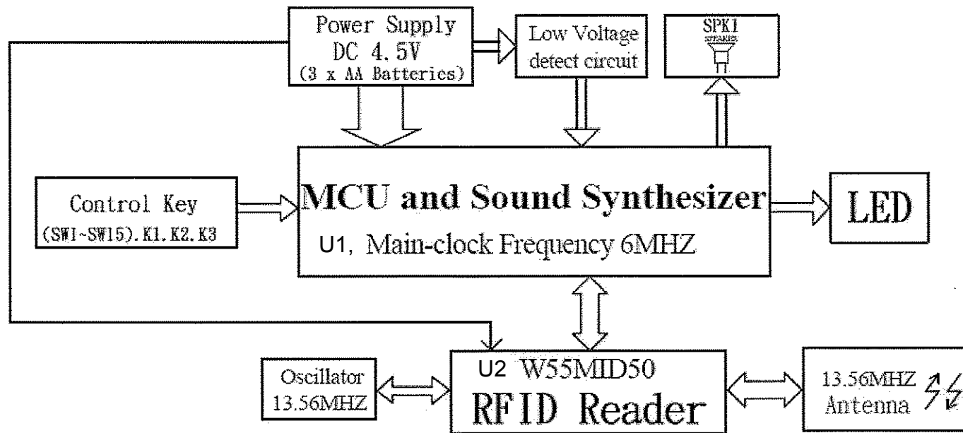
Little Tikes Learning Market-cashier Functional Block Diagram
