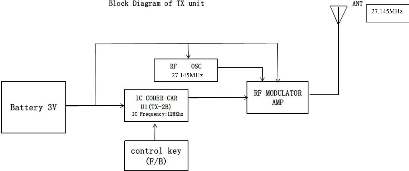
Block Diagram of TX unit
