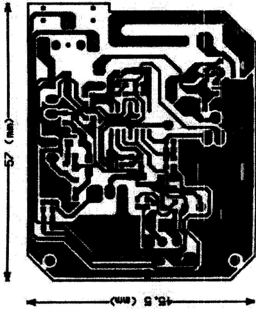
CEM-1 AU 45.5mm x 57mm 1.6mm
