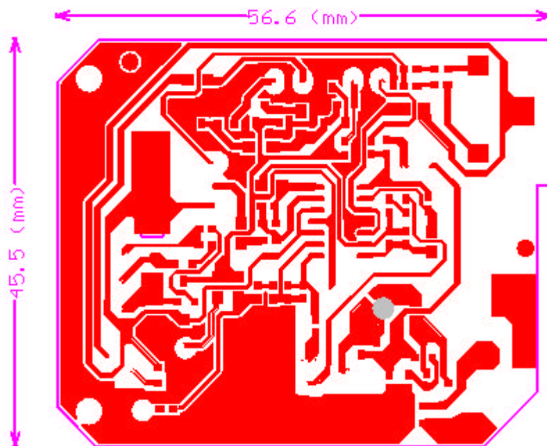
CEM-1 AU 45.5*56.6*1.6mm
