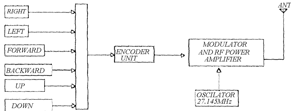
FUNCTION BLOCK DIAGRAM
