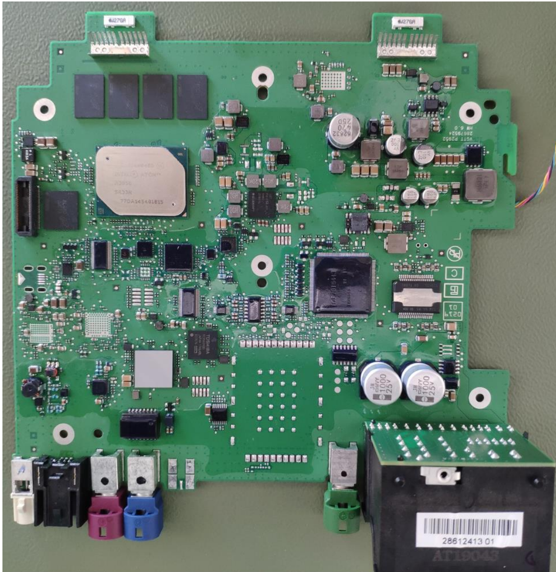
Figure 11 – SEM HIGH DAB PCB - Board Top View
