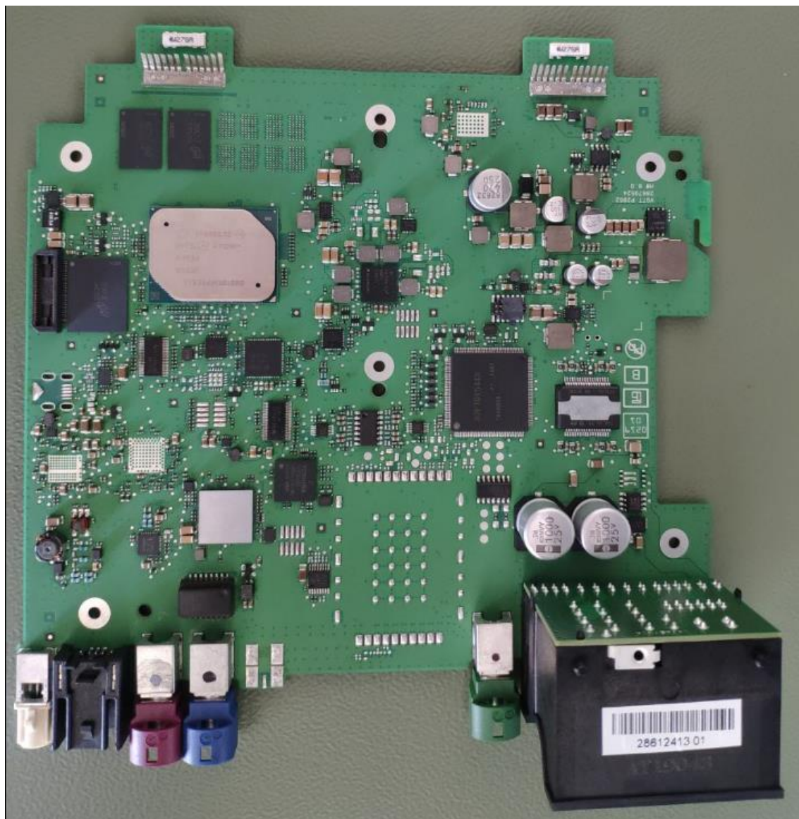
Figure 13 – SEM LOW DAB - PCB Top View
