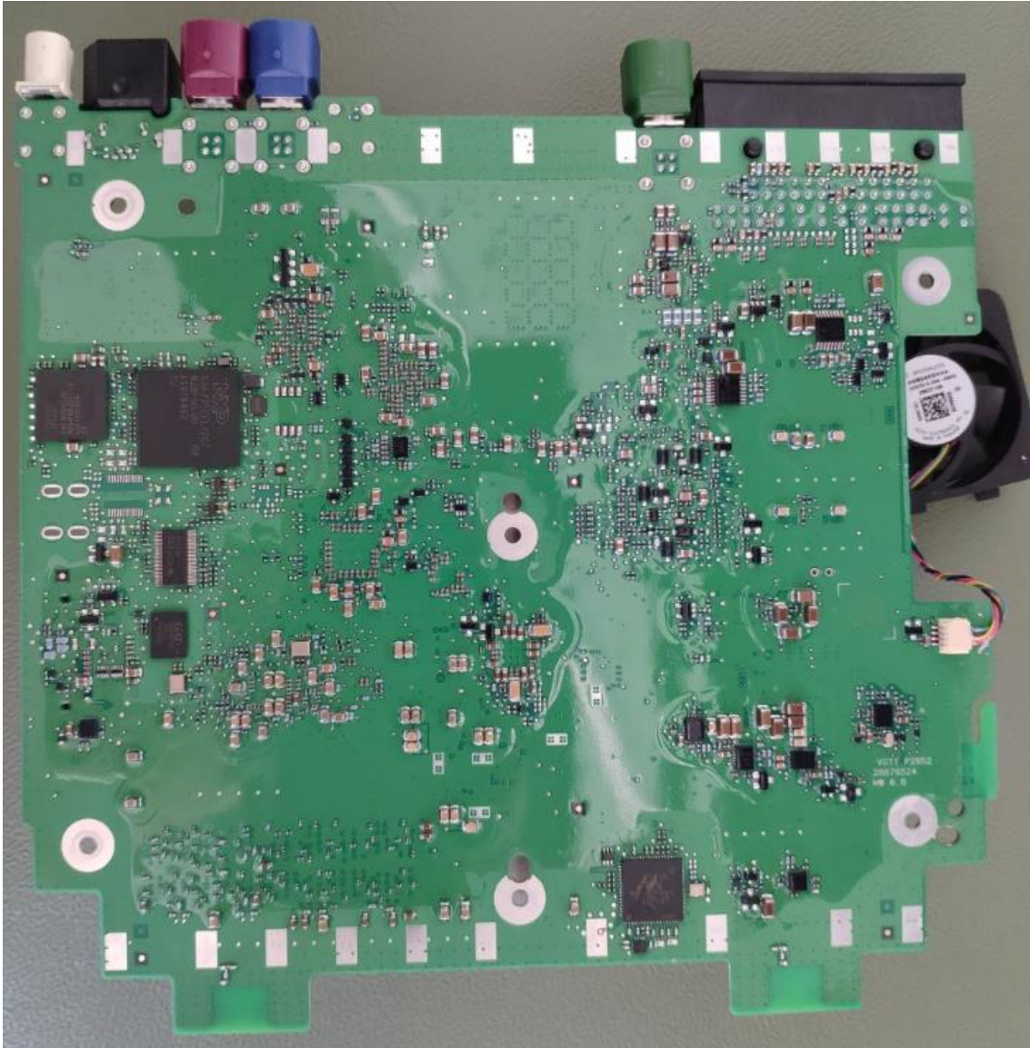
Figure 12 – SEM HIGH DAB - PCB Bottom View
