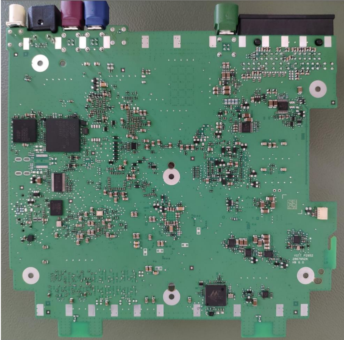
Figure 14 - SEM LOW DAB - PCB Bottom View
