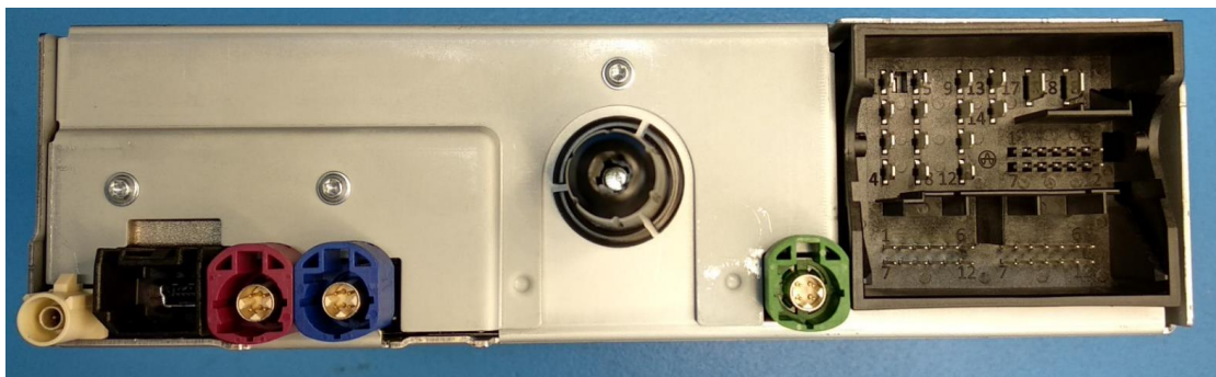
Figure 2 - SEM rear picture
