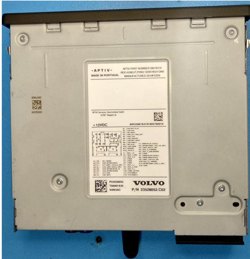
Figure 5 – SEM Top View
