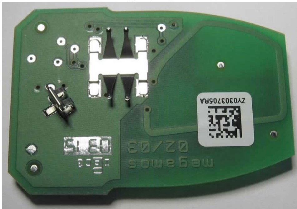
Internal Photos Back view PCB
