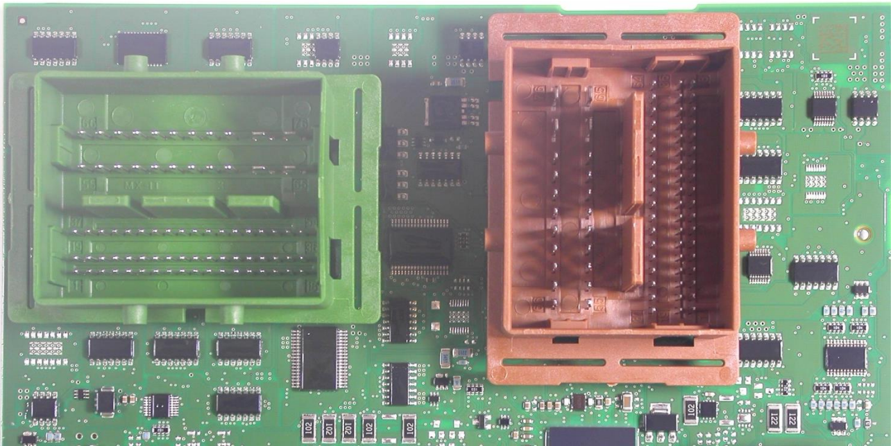
Circuit board 1:
