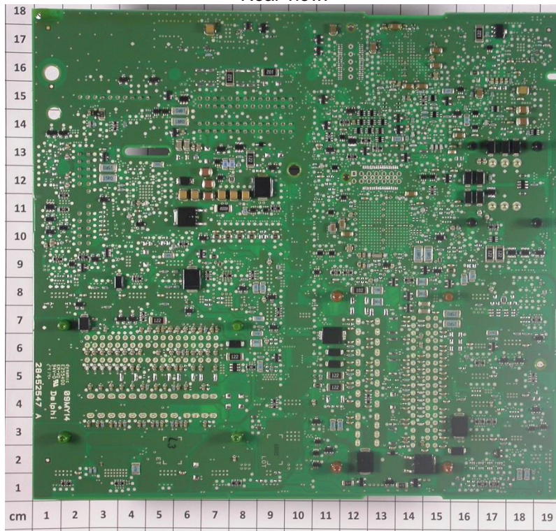
Rear view:
