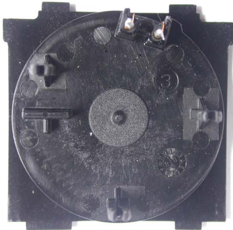
Internal Photo Transceiver coil: Bottom view
