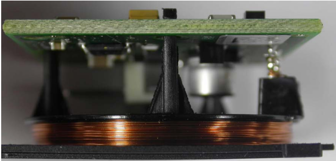
Internal Photo PCB with Transceiver coil Side view
