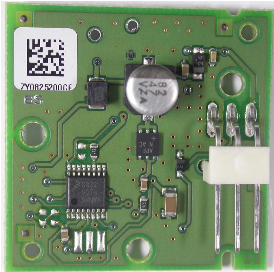
Internal Photo PCB without Transceiver coil Top view
