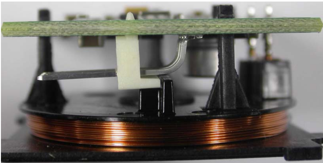
Internal Photo PCB with Transceiver coil Side view
