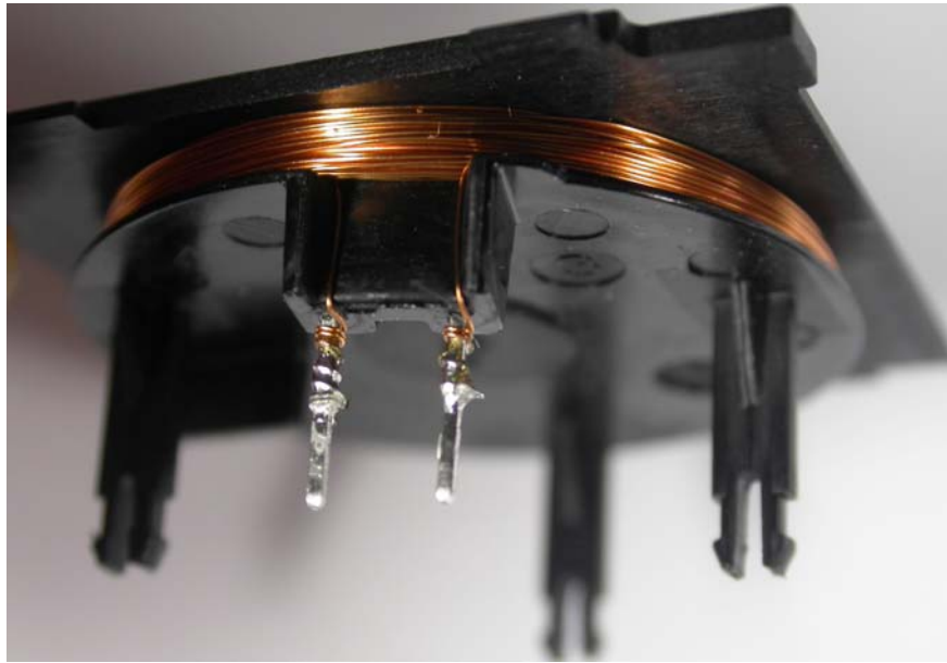
Internal Photo Transceiver coil Side view
