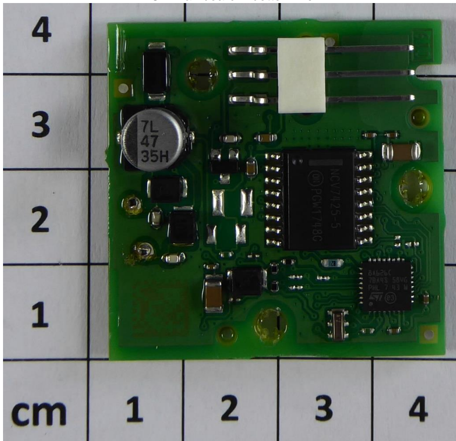
PCB mainboard – bottom view
