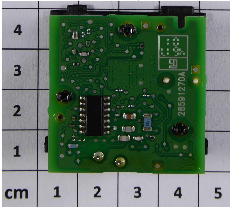
PCB mainboard – bottom view
