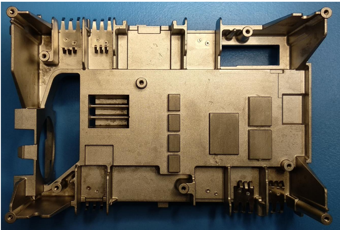
Figure 14 - Heat Sink side that connects with Main Board
