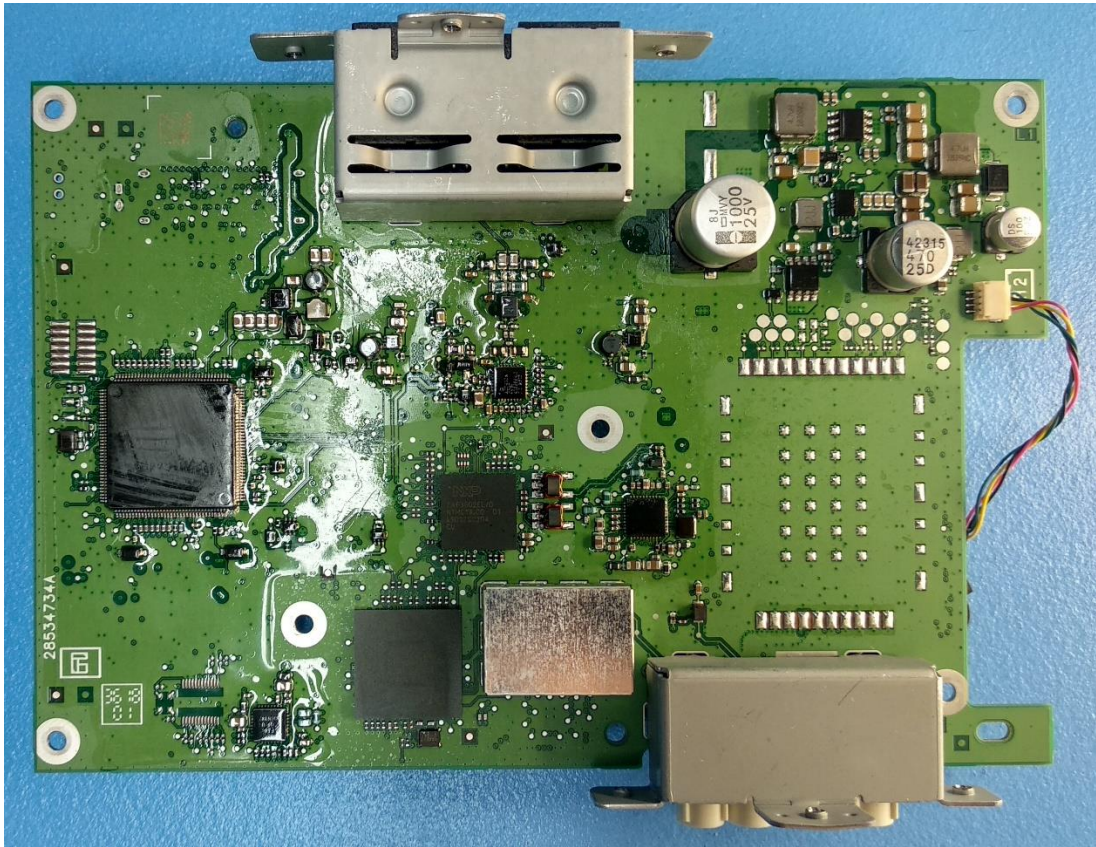
Figure 9 – IHU 4.0 HIGH DAB - Tuner Board Top View
