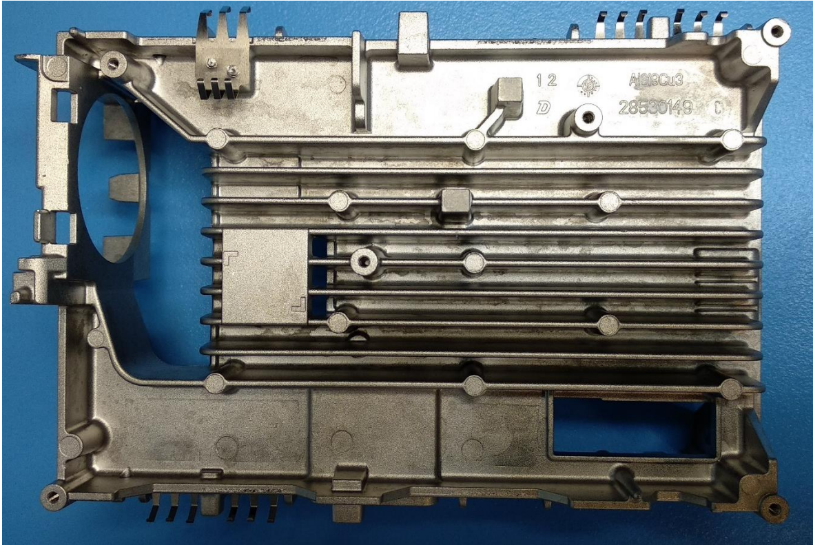
Figure 13 - Heat Sink side that connects with the Tuner Board
