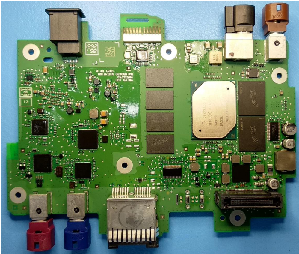
Figure 11 - IHU 4.0 HIGH DAB - Main Board Top View
