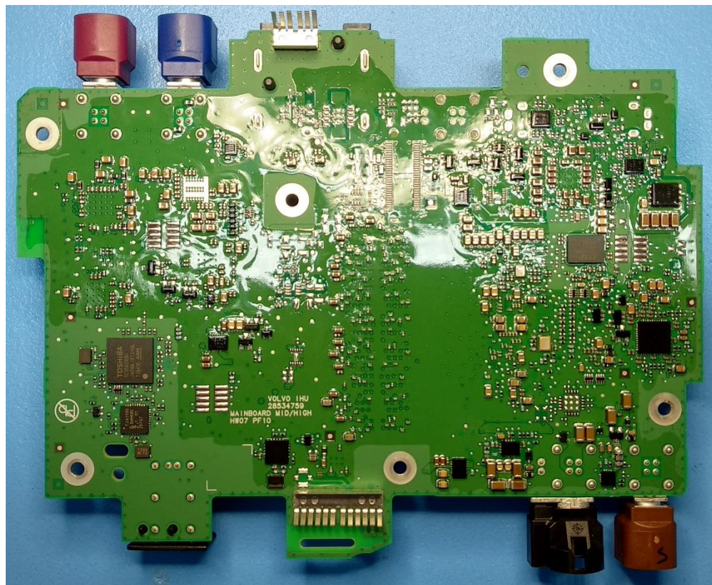
Figure 12 - IHU 4.0 HIGH DAB - Main Board Bottom View
