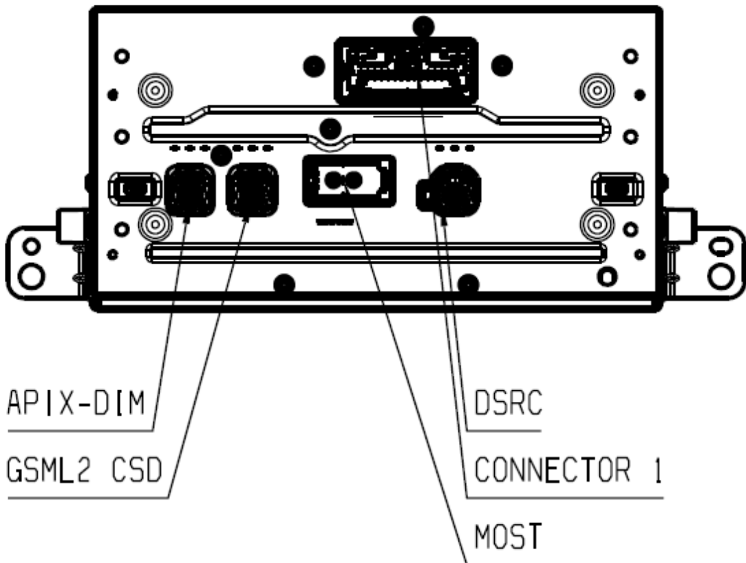
Figure 4 - IHU 4.0 side facing front of the Car, Drawing with Connectors Description
