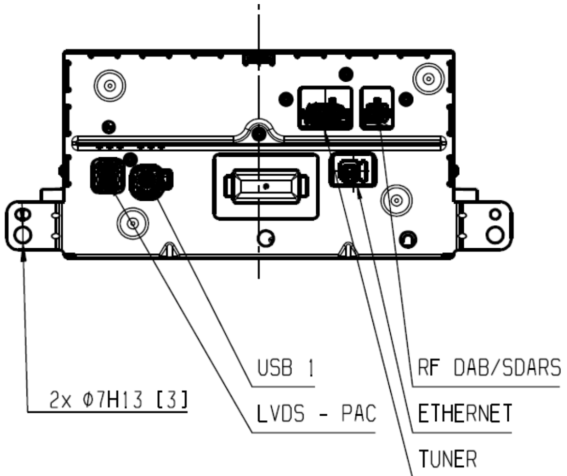
Figure 2 - IHU 4.0 side facing the rear of the Car, Drawing with Connectors Description
