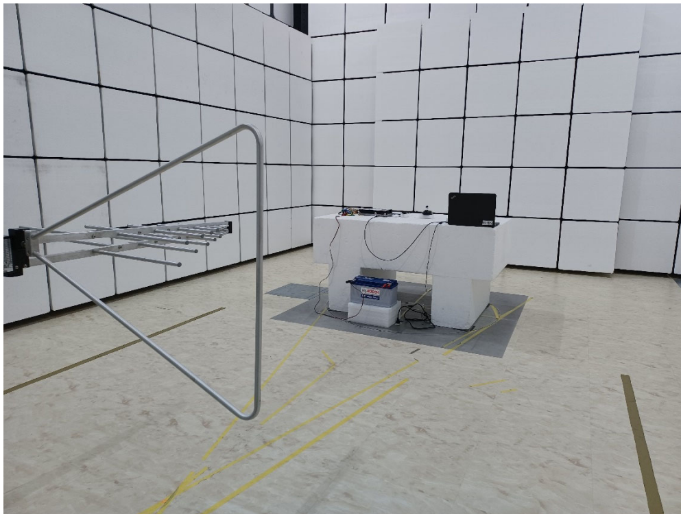
Radiated Test
