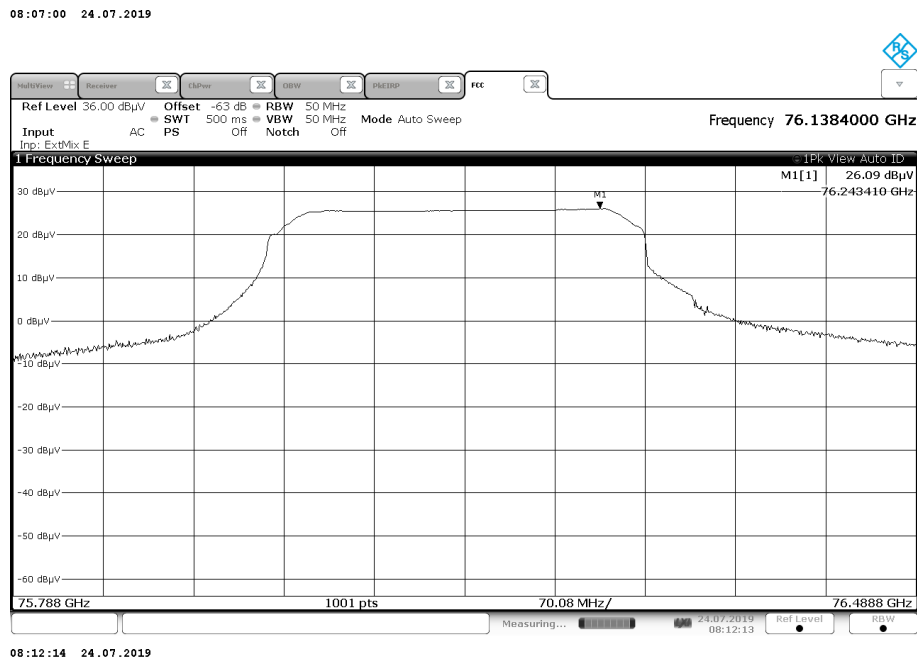
175 MHz, Lowest Channel
