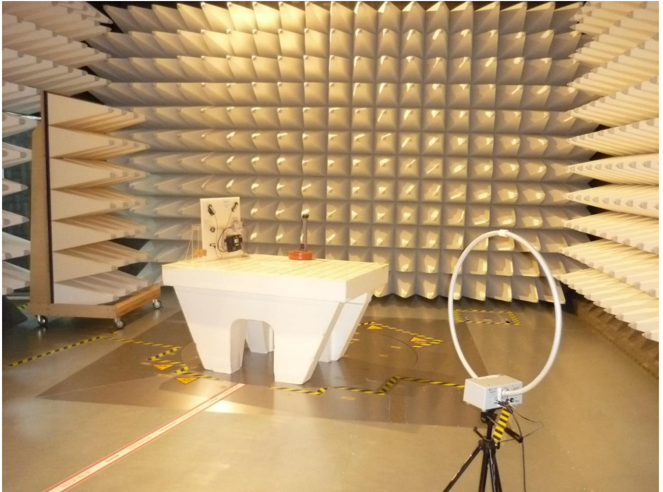
Tested frequency range 9 kHz – 30 MHz
