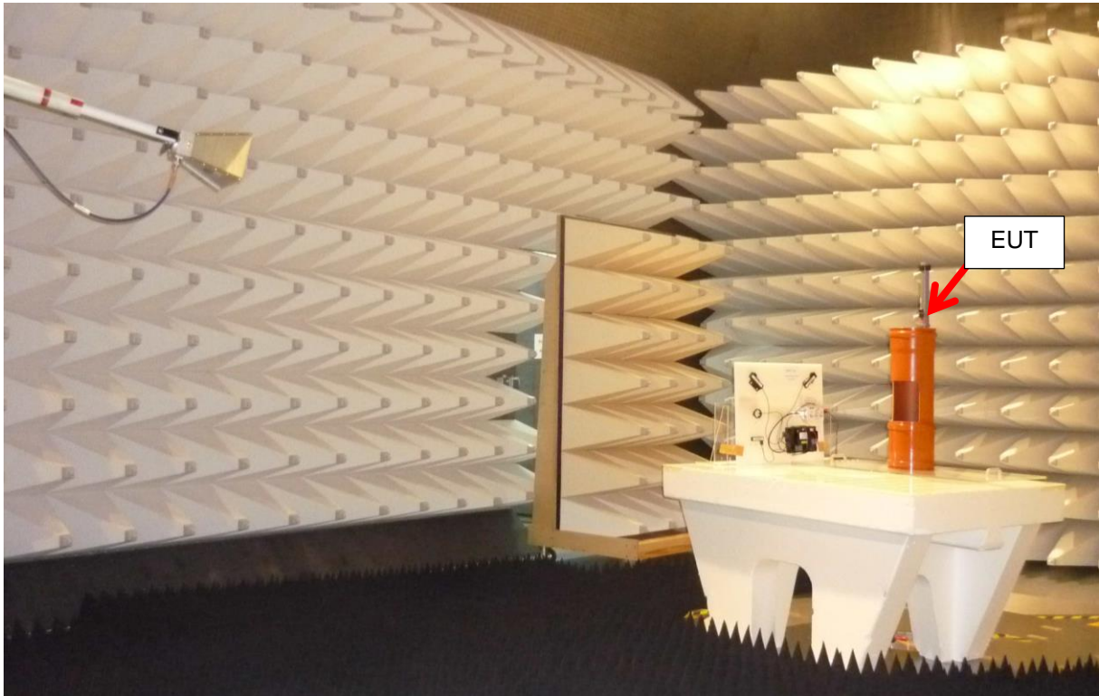
Tested frequency range > 1 GHz
